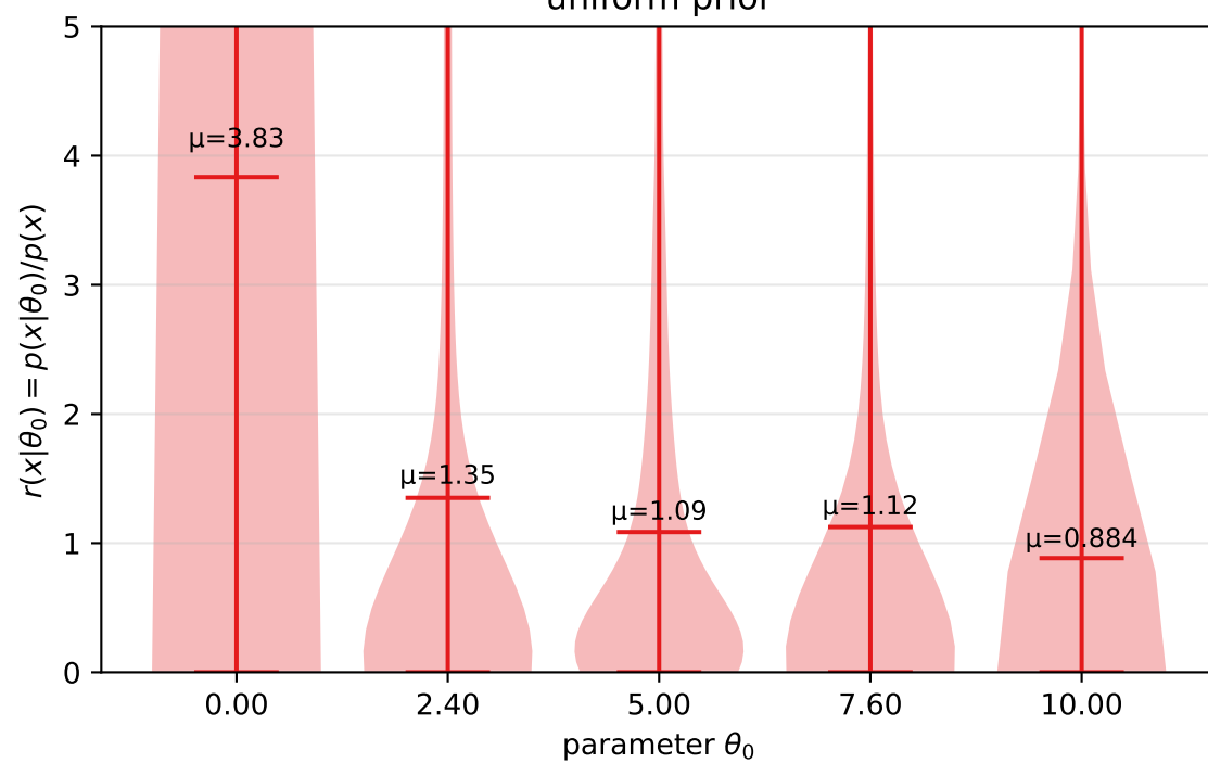
uniform prior
