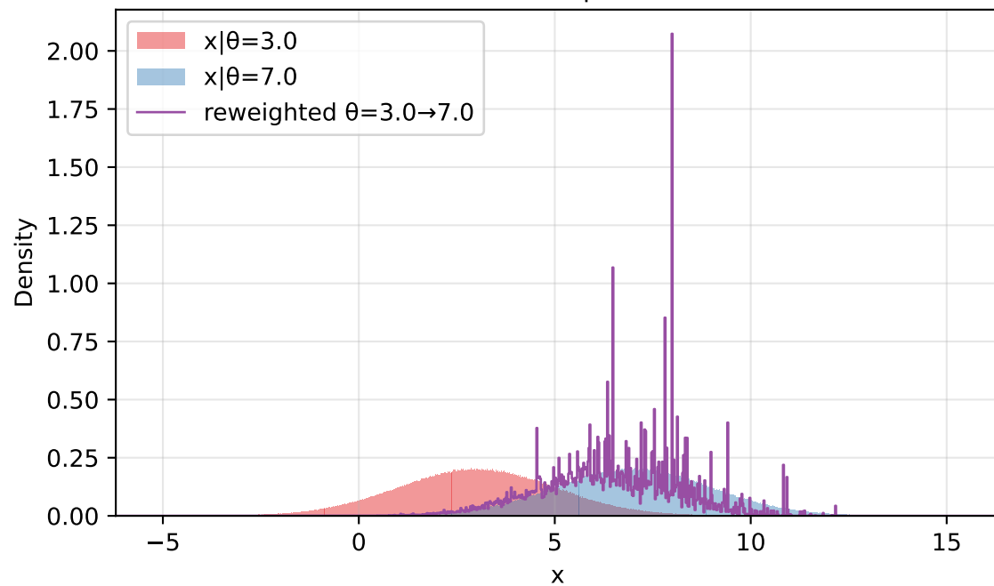
grid prior N=1,000,000 | ESS=348
