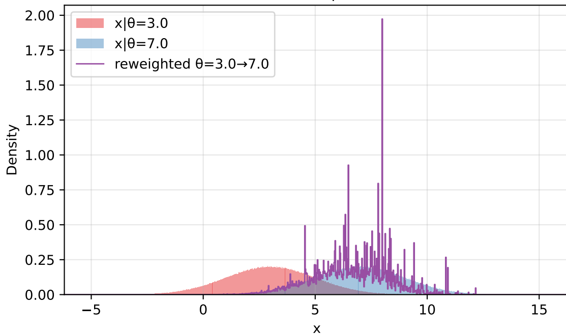
exponential prior N=1,000,000 | ESS=316
