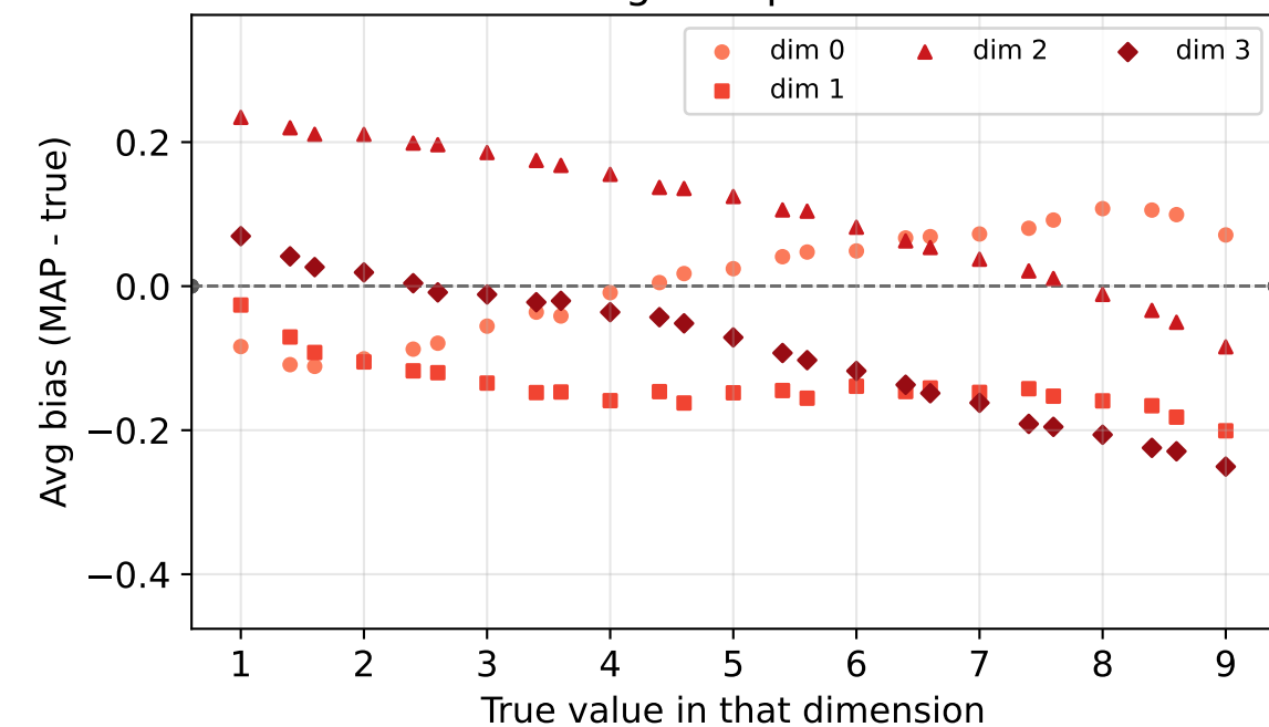
exponential: avg bias per dimension
