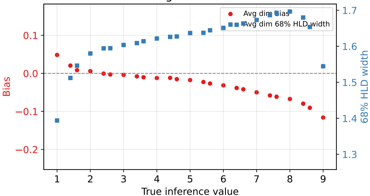
exponential: averages across dimensions
