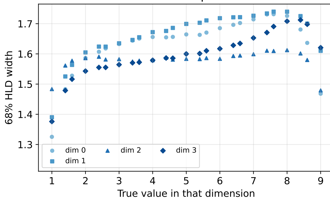
exponential: HLD width per dimension
