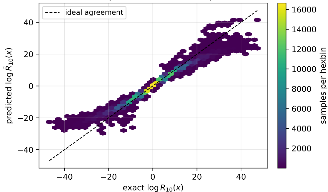
uniform prior pooled RMSE=1.93 | pair median=0.867 | pair worst=7.94
