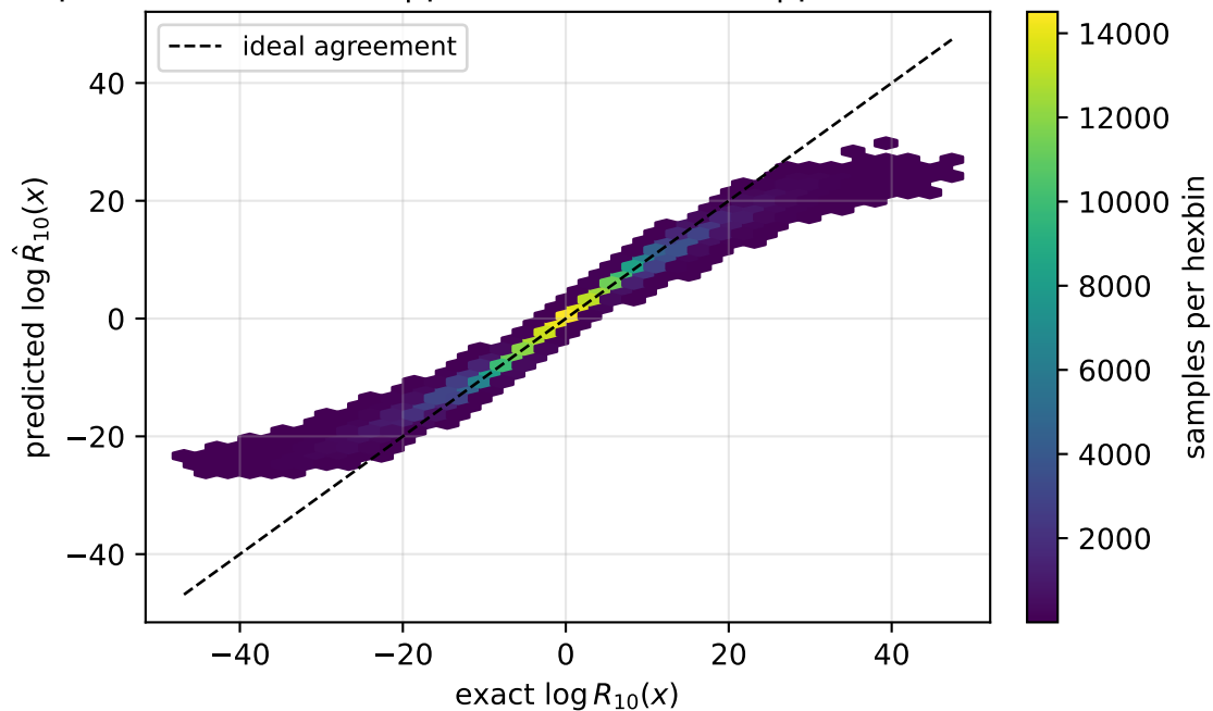
grid prior pooled RMSE=1.82 | pair median=0.886 | pair worst=7.37
