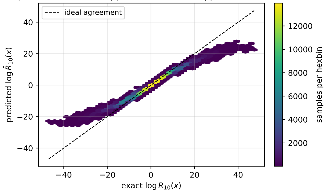
exponential prior pooled RMSE=2.34 | pair median=1.21 | pair worst=8.54
