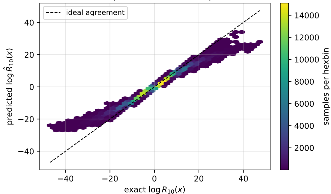
normal prior pooled RMSE=2.17 | pair median=1.16 | pair worst=8.16
