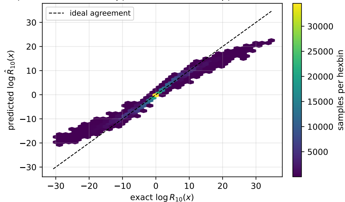
grid prior pooled RMSE=0.93 | pair median=0.487 | pair worst=4.12
