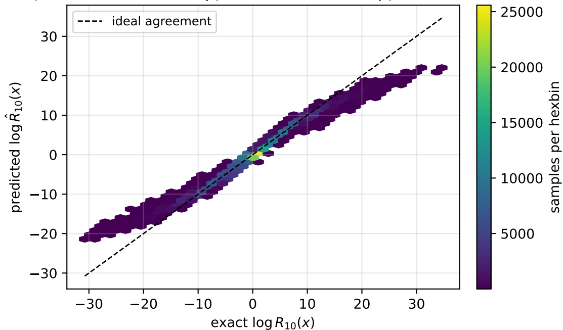
exponential prior pooled RMSE=0.785 | pair median=0.468 | pair worst=3
