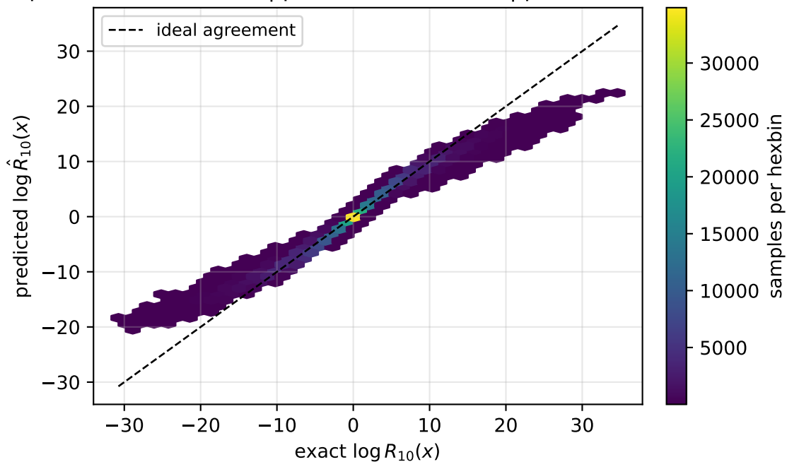
normal prior pooled RMSE=0.978 | pair median=0.553 | pair worst=3.84
