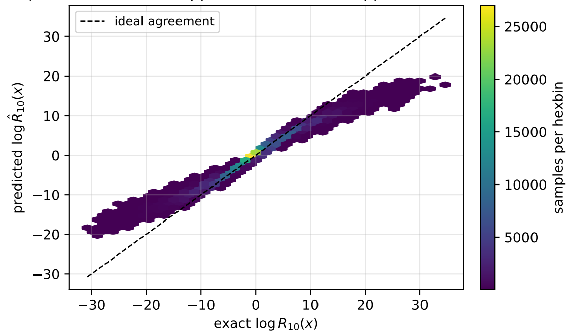
uniform prior pooled RMSE=1.41 | pair median=0.675 | pair worst=5.07
