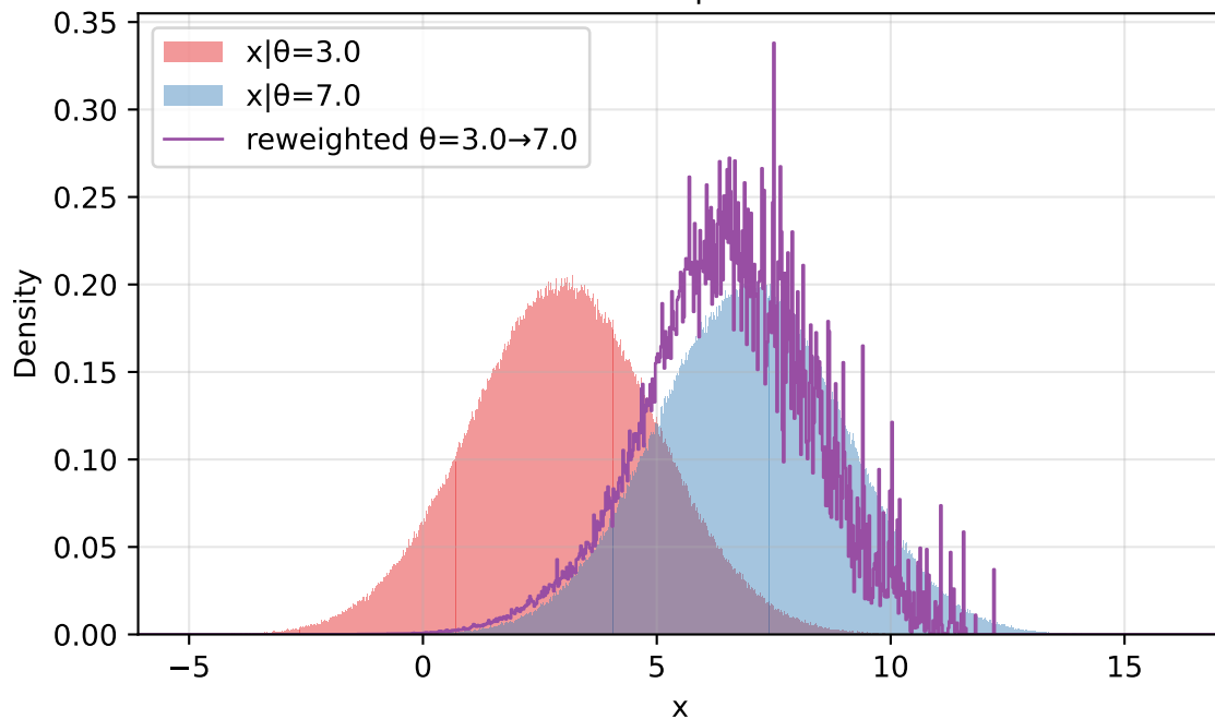
exponential prior N=1,000,000 | ESS=3,165
