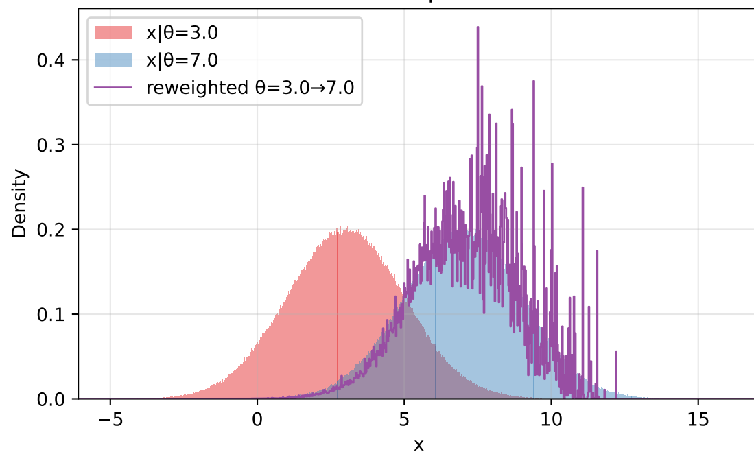
grid prior N=1,000,000 | ESS=3,181
