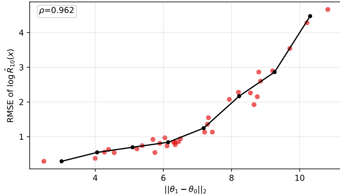
uniform prior median=0.955 | worst=4.66
