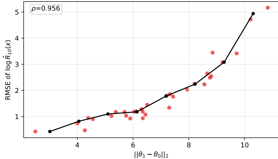
normal prior median=1.31 | worst=5.16
