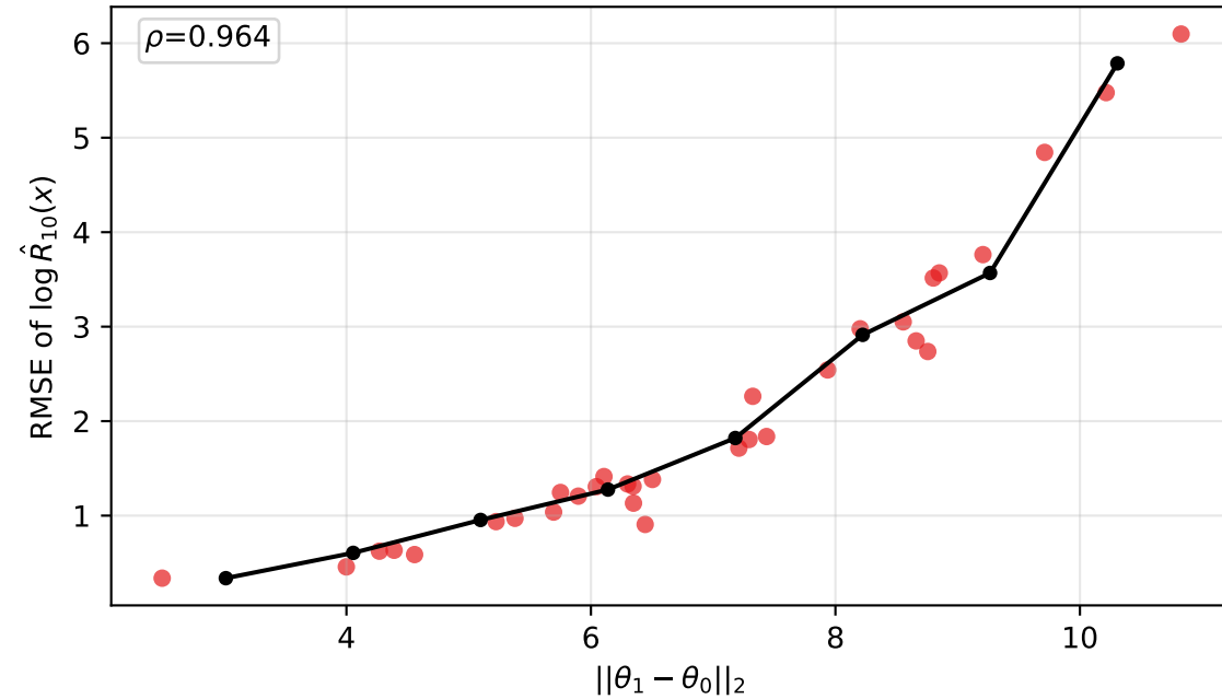
exponential prior median=1.4 | worst=6.1
