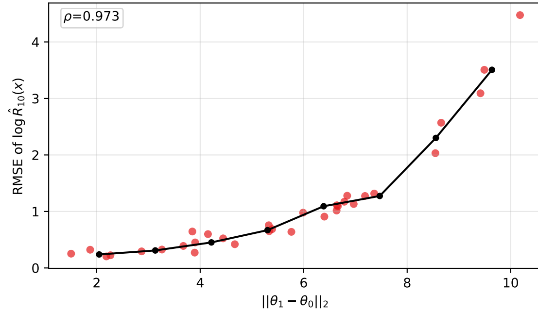
normal prior median=0.722 | worst=4.48
