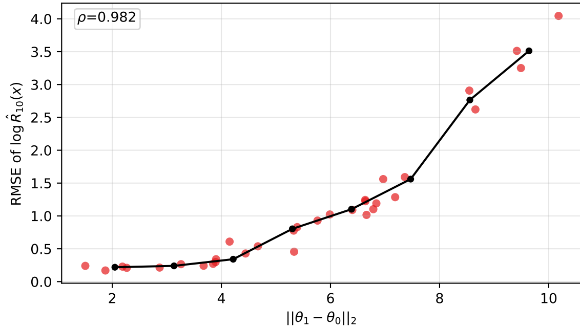
uniform prior median=0.88 | worst=4.04
