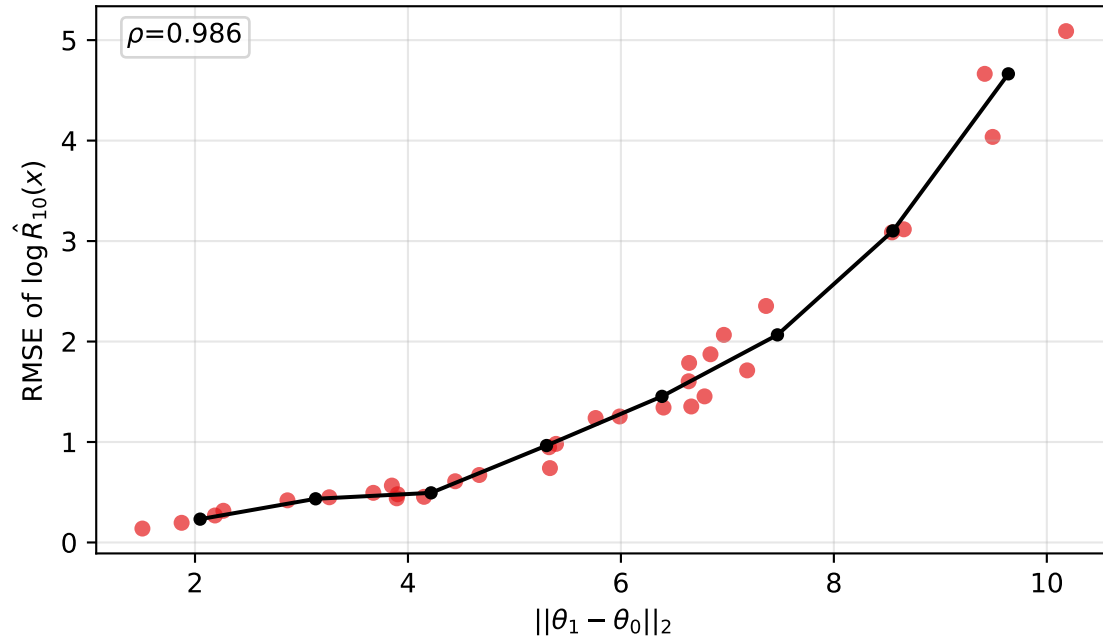
exponential prior median=1.11 | worst=5.09
