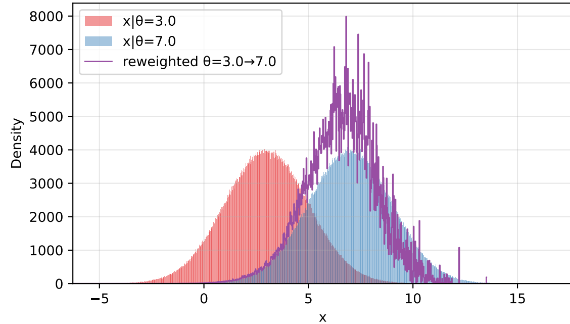
uniform prior N=1,000,000 | ESS=6,584
