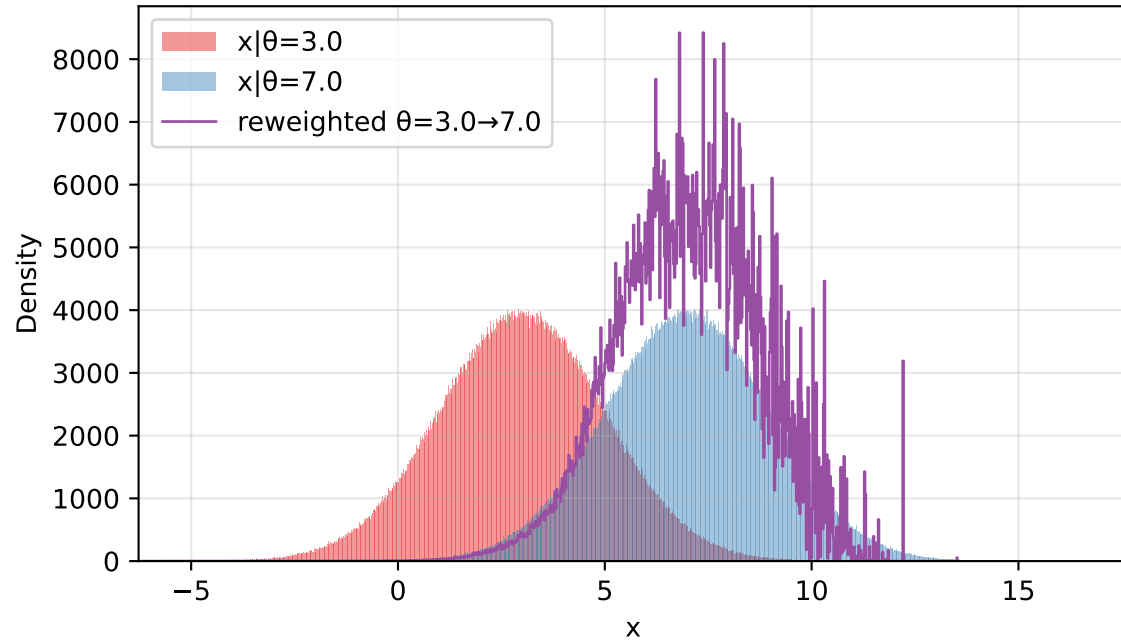
normal prior N=1,000,000 | ESS=4,910
