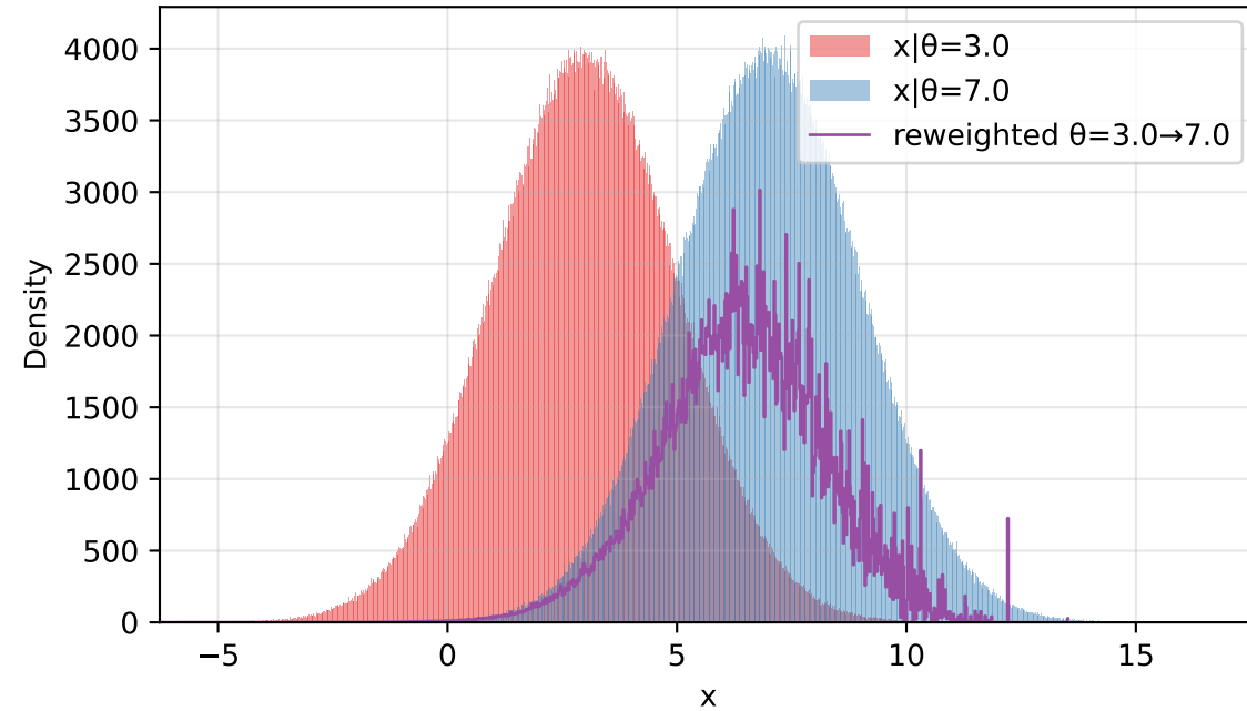
exponential prior N=1,000,000 | ESS=8,333
