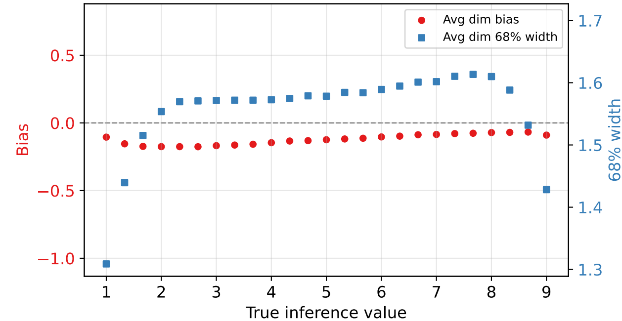
exponential: averages across dimensions
