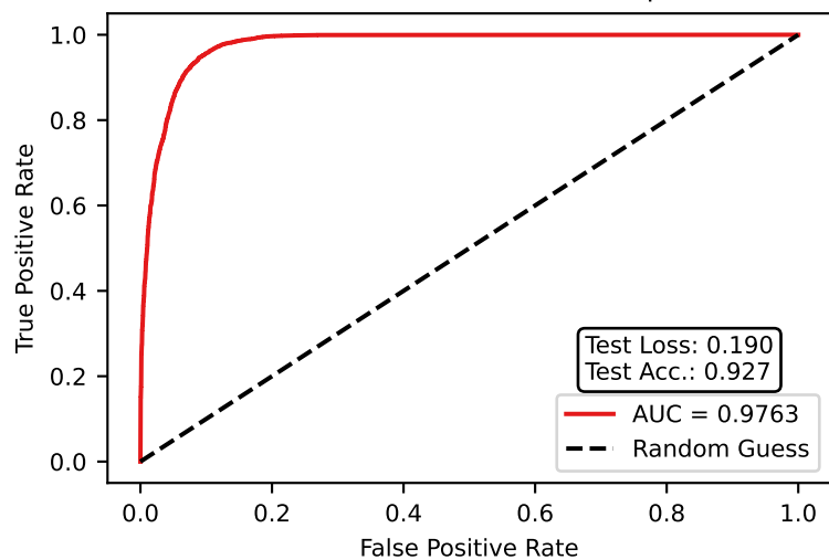
Test ROC Curve for 0. normal prior
