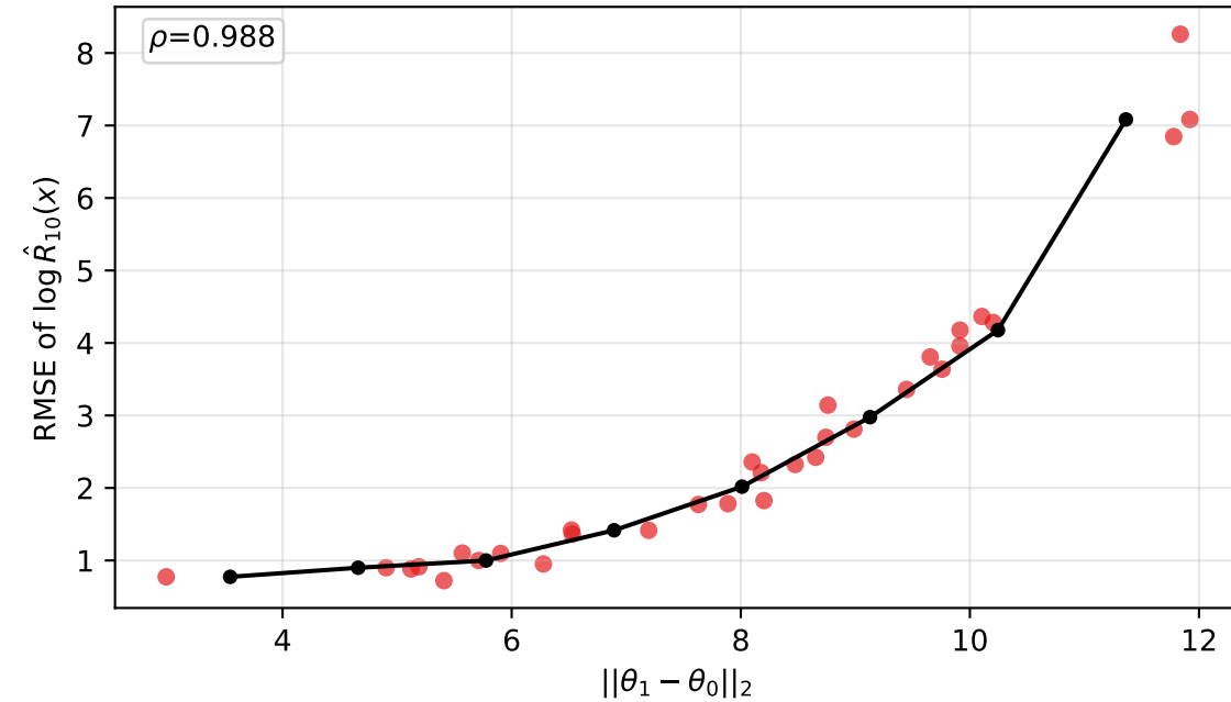
exponential prior median=2.27 | worst=8.26
