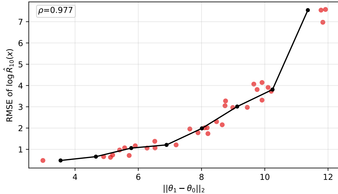
normal prior median=2.01 | worst=7.58
