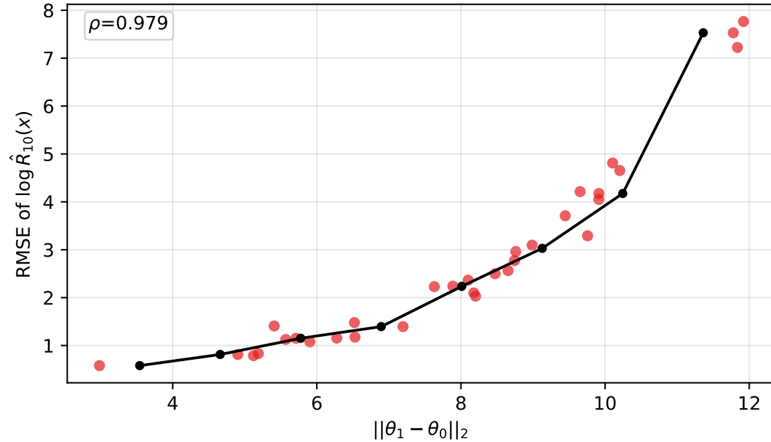
uniform prior median=2.3 | worst=7.76
