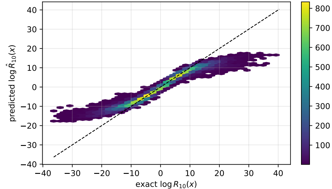
exponential prior
