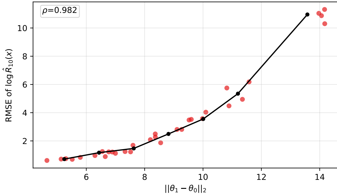
normal prior median=2.18 | worst=11.3
