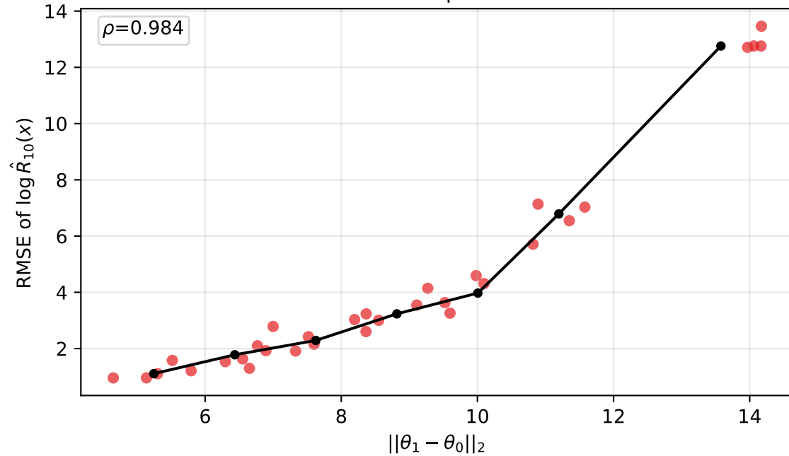
exponential prior median=3.02 | worst=13.5
