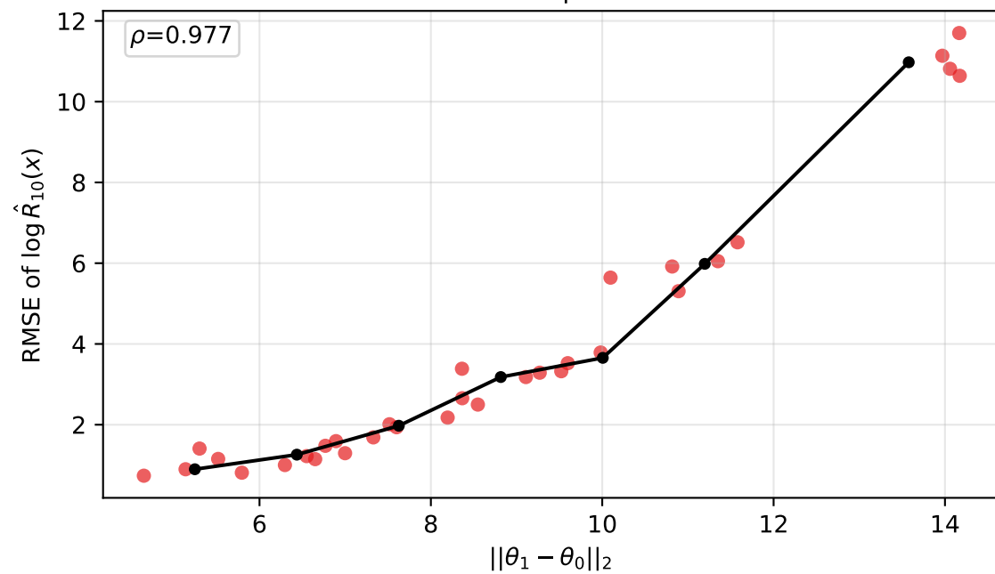
uniform prior median=2.58 | worst=11.7
