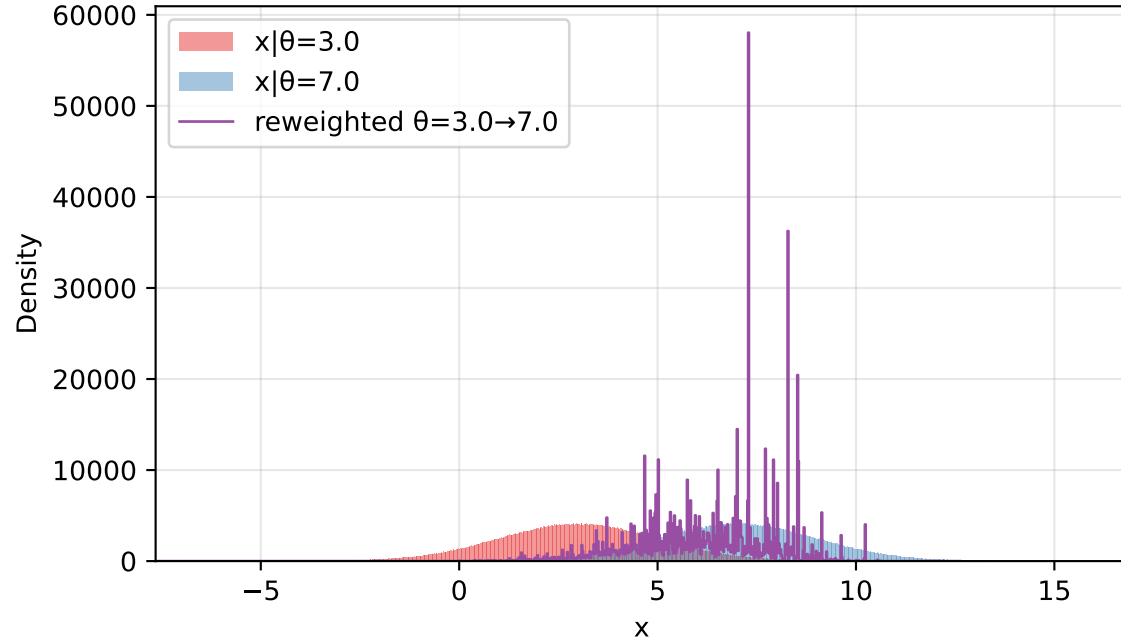
normal prior N=1,000,000 | ESS=90
