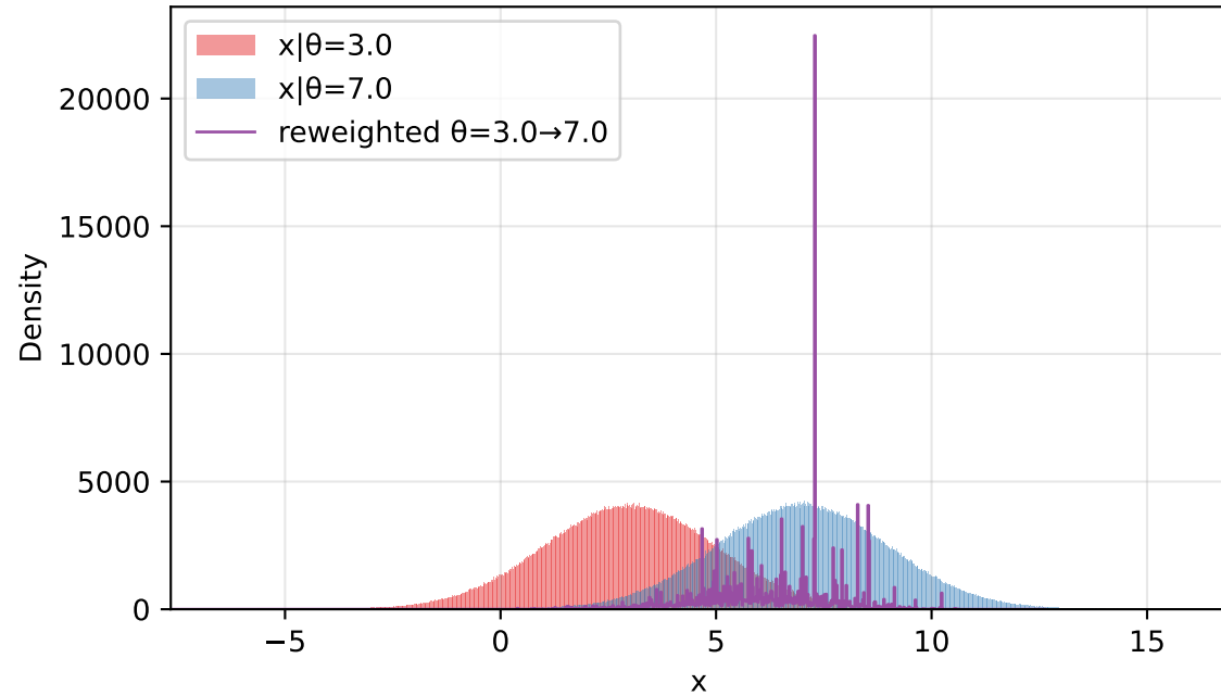
uniform prior N=1,000,000 | ESS=43
