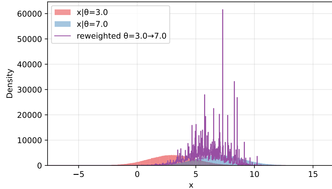
exponential prior N=1,000,000 | ESS=231
