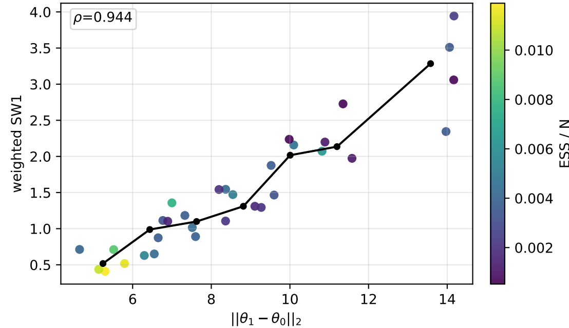
normal prior median=1.33 | worst=3.94
