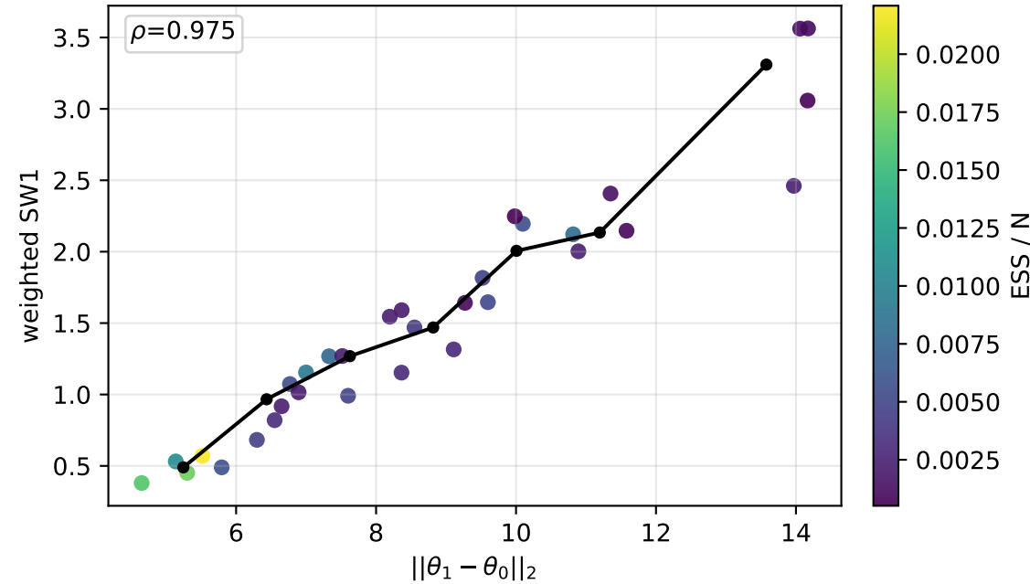
uniform prior median=1.39 | worst=3.56
