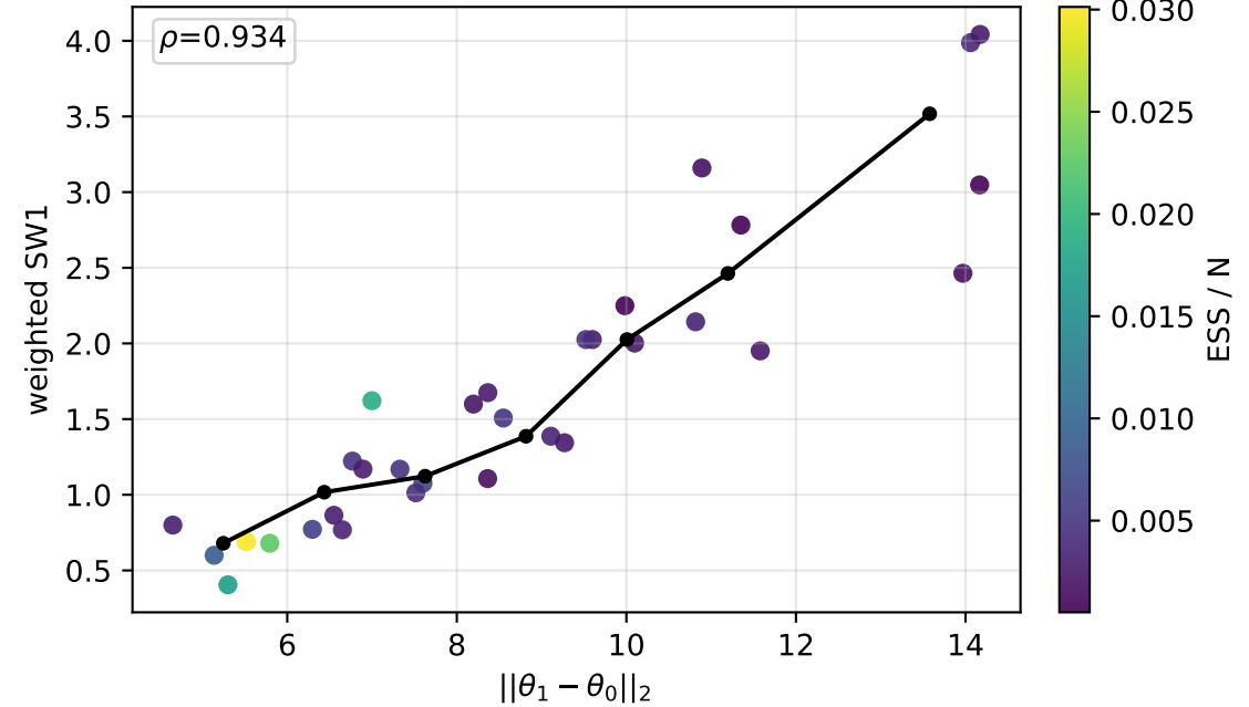
exponential prior median=1.45 | worst=4.04
