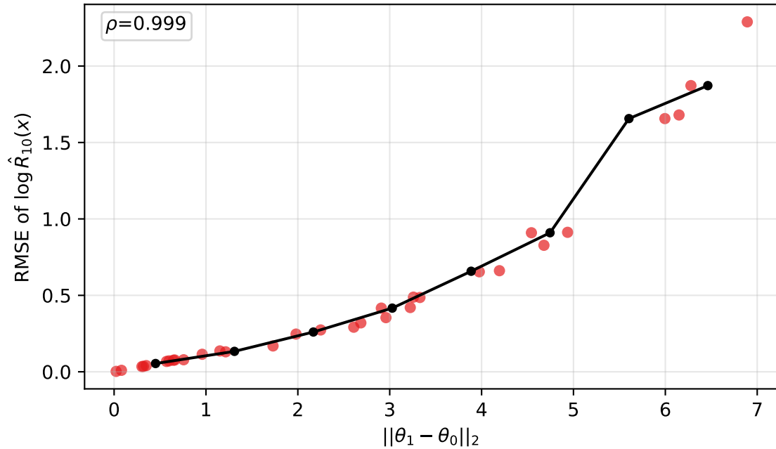
normal prior median=0.283 | worst=2.29
