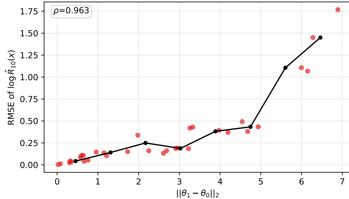
uniform prior median=0.16 | worst=1.77
