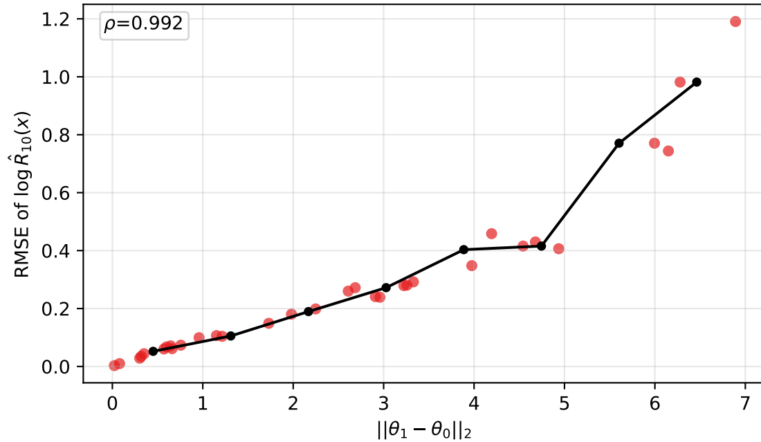
exponential prior median=0.219 | worst=1.19
