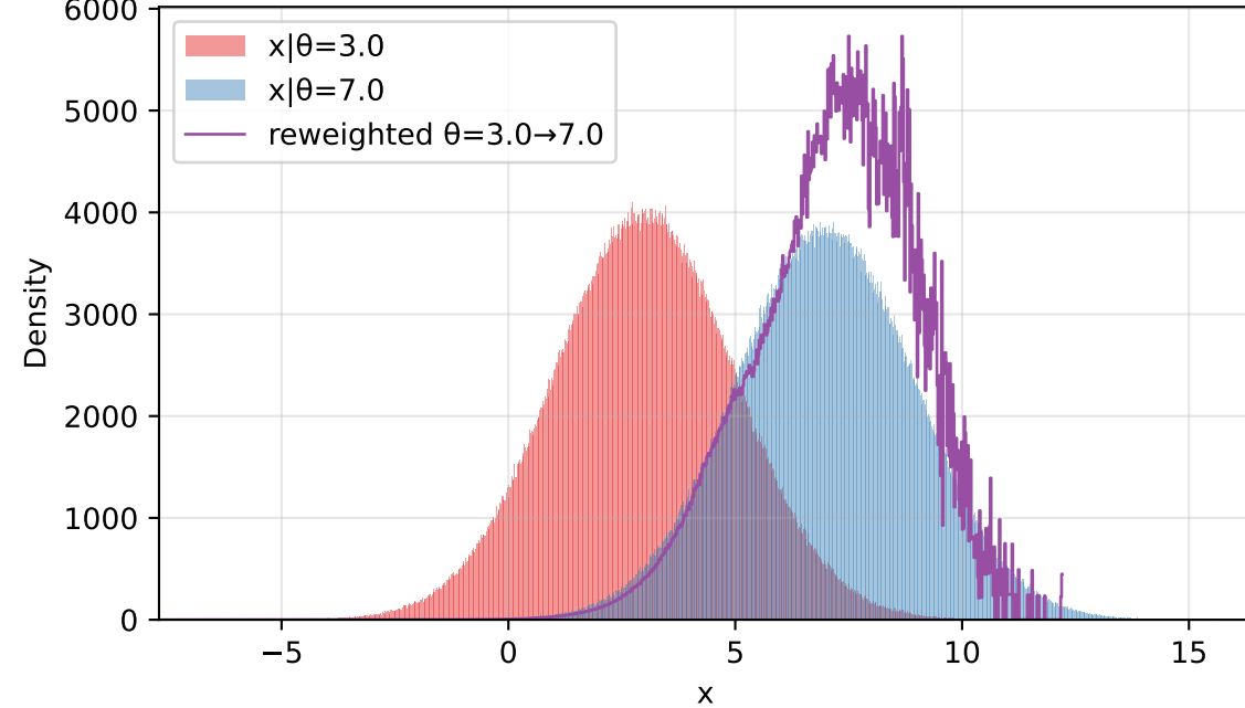
exponential prior N=1,000,000 | ESS=31,277
