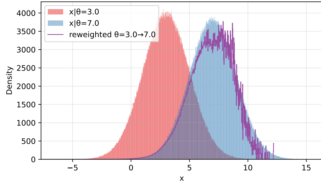
uniform prior N=1,000,000 | ESS=44,085
