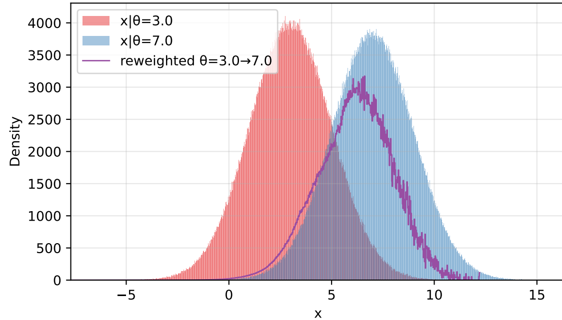
normal prior N=1,000,000 | ESS=126,785
