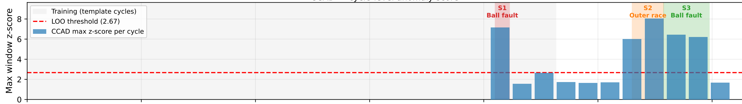
CCAD — cycle-level anomaly score
