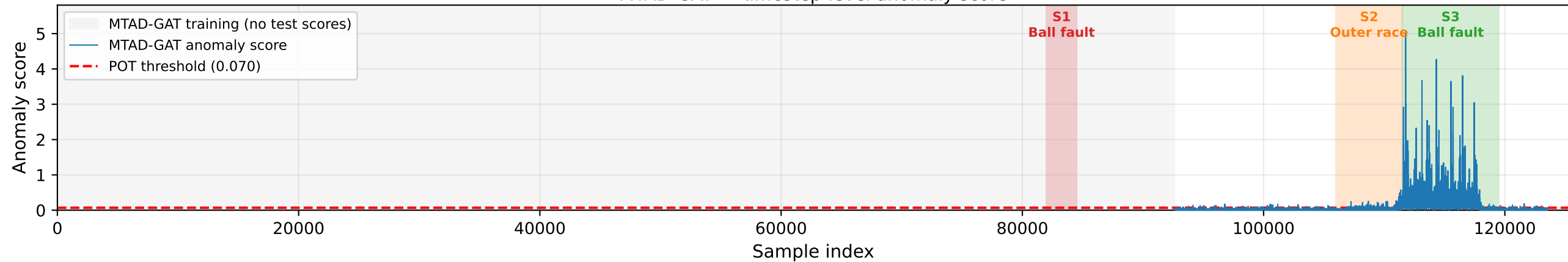
MTAD-GAT — timestep-level anomaly score
