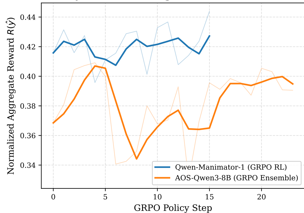
GRPO Policy Reward Convergence (AST + CE Executability) Policy Gradient Loss Dynamics under \varepsilon = 0.2 Clipping
