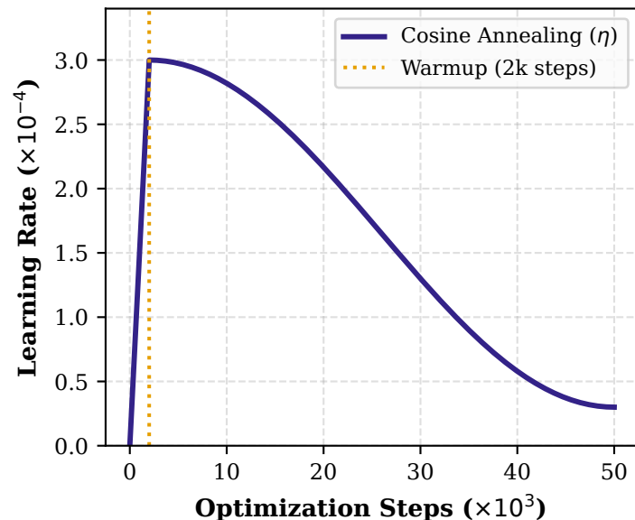
(c) Learning Rate Schedule
