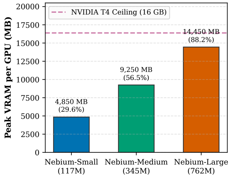
(b) Peak Memory Footprint
