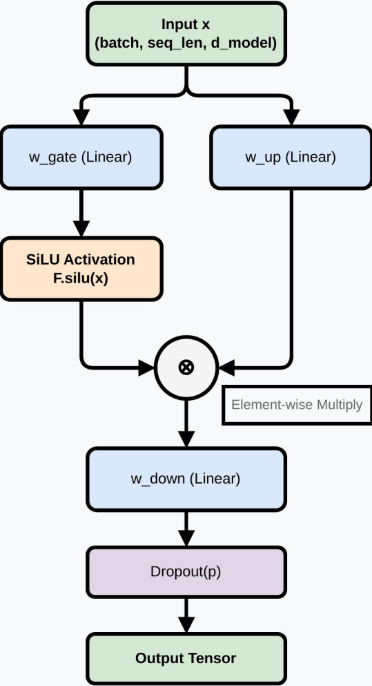
SwiGLU Architecture
