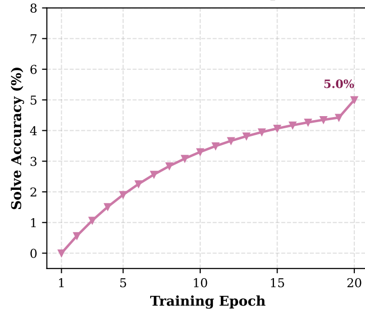
(f) Puzzles 2000+ Elo (Expert Tier)
