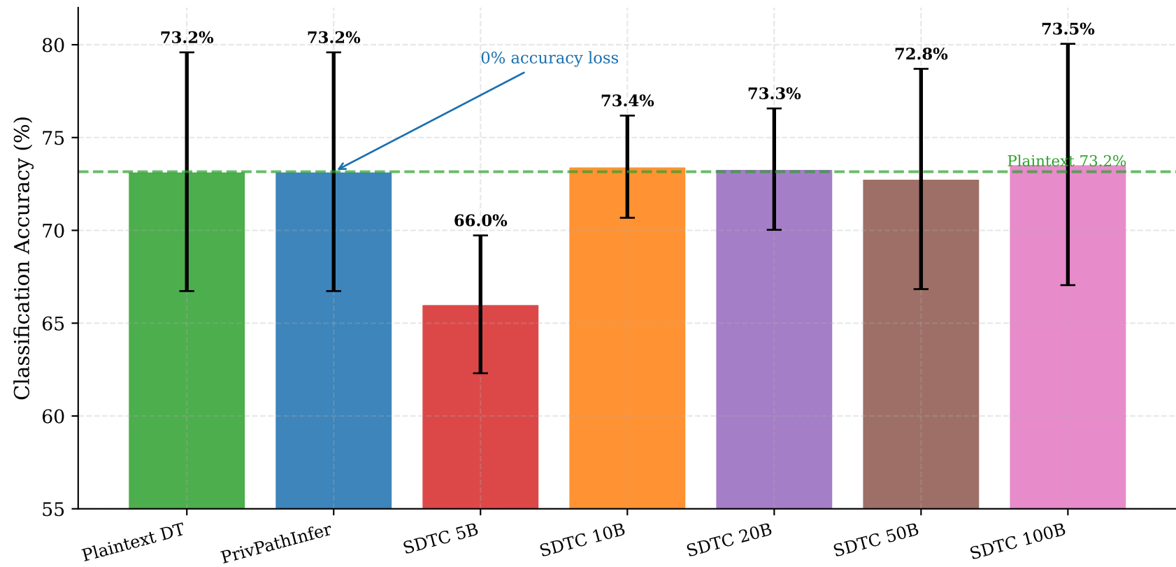
Figure 1: Accuracy Comparison — PrivPathInfer vs SDTC (PIMA Diabetes, 5-fold CV, max_depth=5)
