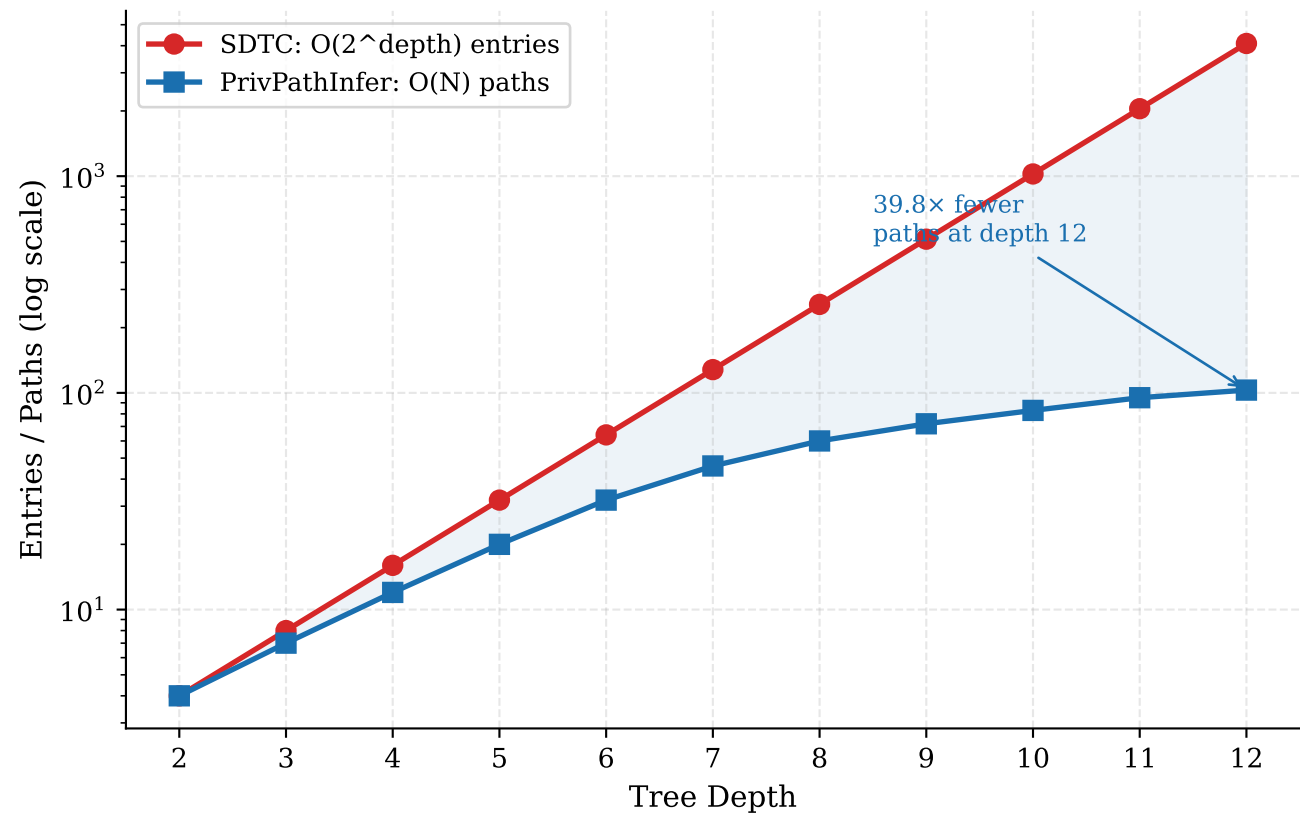
Figure 2: Storage — Entry/Path Count (PrivPathInfer O(N) vs SDTC O(2^N) )
