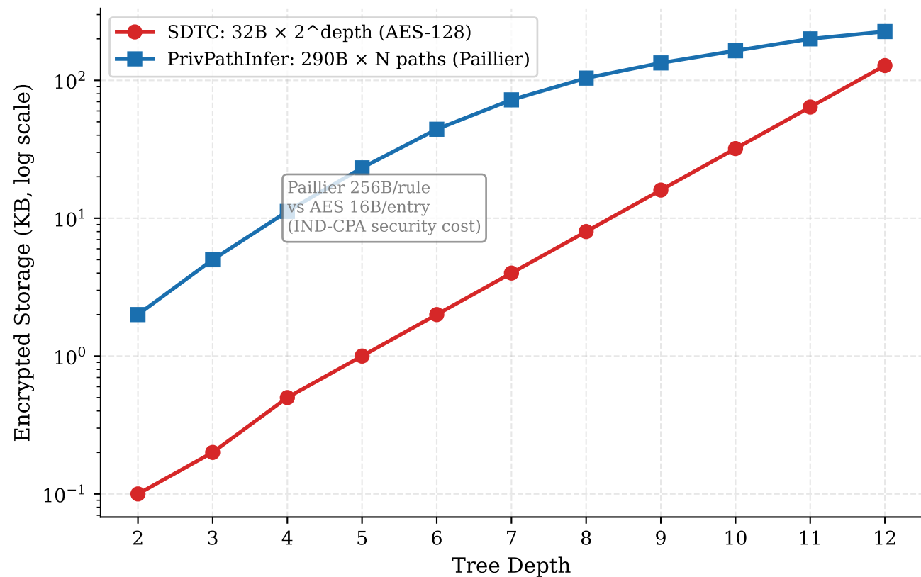
Figure 3: Storage — Encrypted Bytes (Paillier IND-CPA overhead vs AES)
