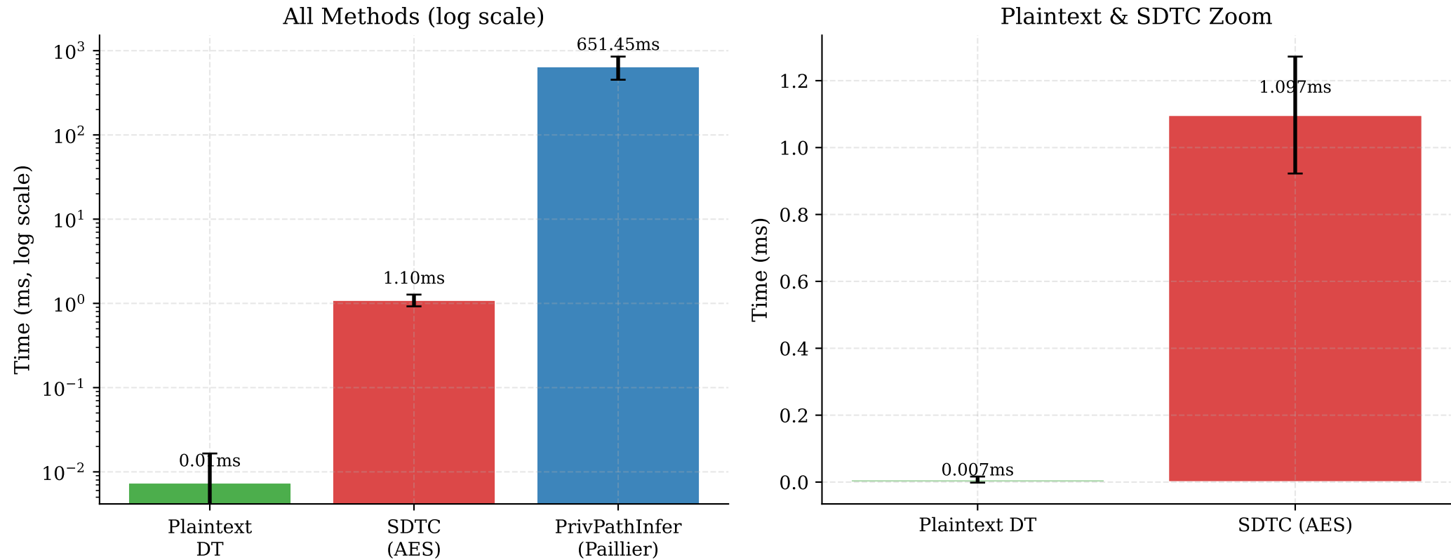
Figure 4: Per-Query Inference Time (1024-bit Paillier, PIMA dataset, depth=5, n=100)
