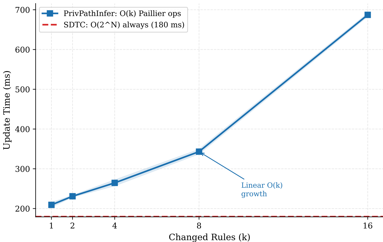
Figure 5: Update Cost — Computation (1024-bit Paillier, PIMA, depth=8)
