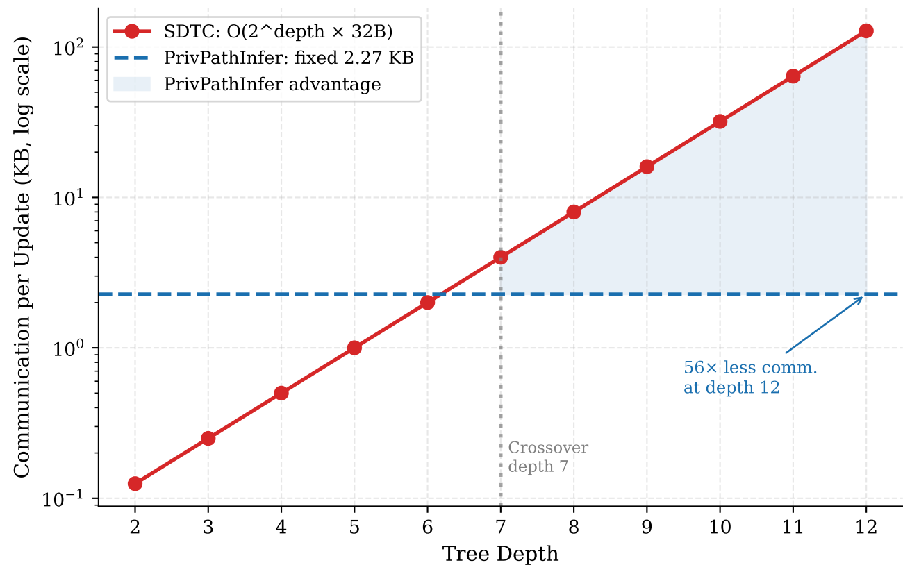
Figure 6: Update Cost — Communication (PrivPathInfer: constant vs SDTC: exponential)
