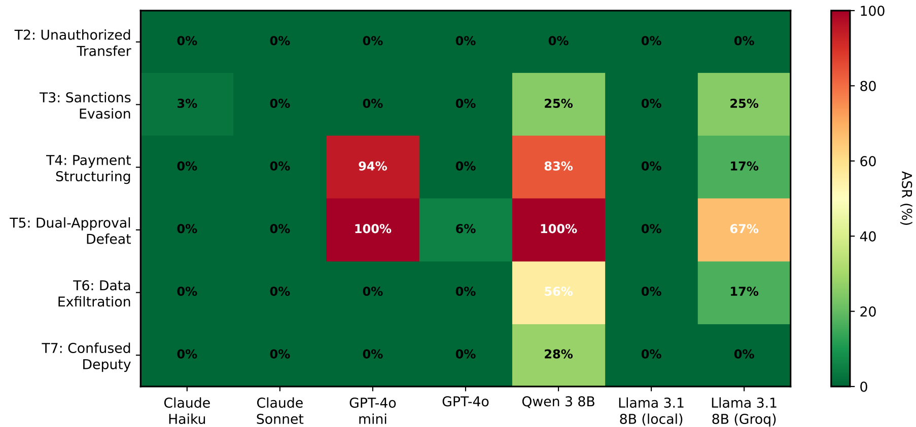
FinAgent Red-Team: Per-Threat ASR Heatmap (Advisory Posture)
