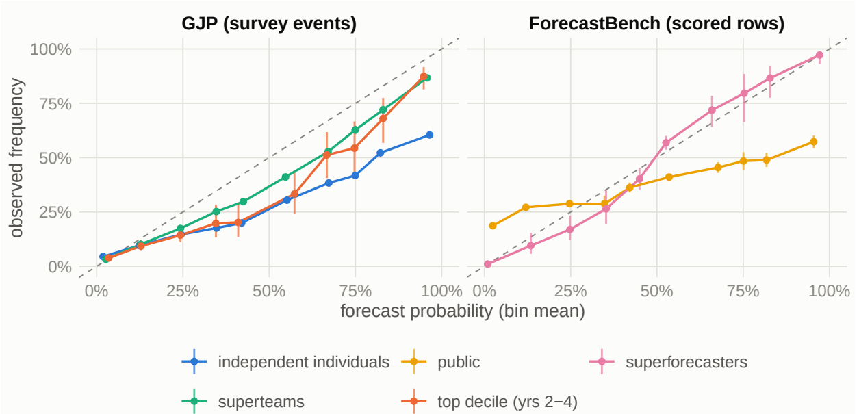
Figure 1: Reliability diagrams, ten equal-width bins, Wilson 95% intervals on the observed frequency. The dashed line is perfect calibration. Points below the line are forecasts that were too high.
