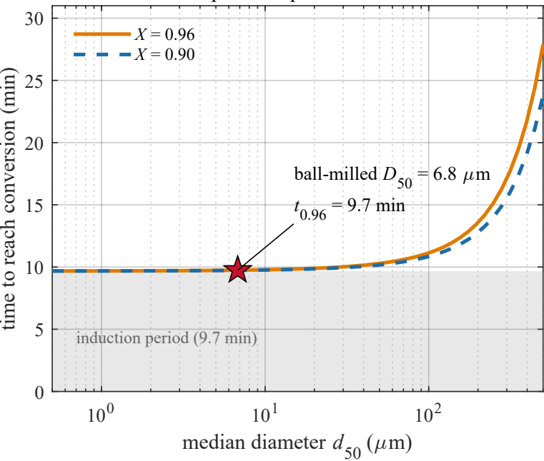
Residence time required vs particle size
