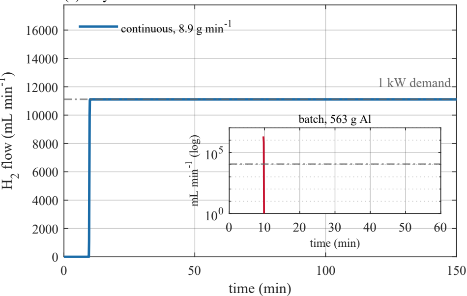
(a) duty control: continuous feed holds demand
