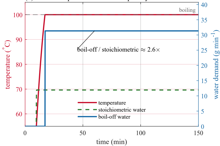
(b) thermal response sets the water penalty
