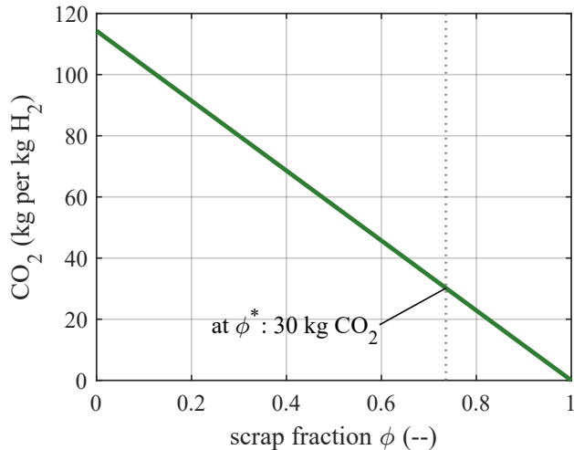
(b) carbon intensity
