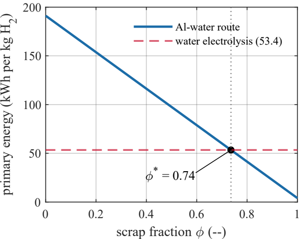
(a) energy break-even
