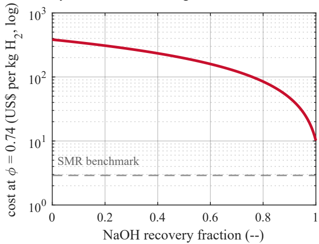
(b) unrecovered NaOH dominates by over an order of magnitude
