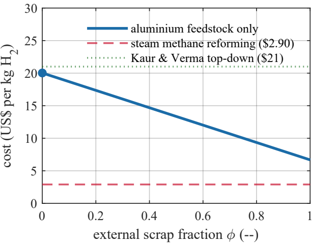
(a) aluminium cost alone is literature-consistent
