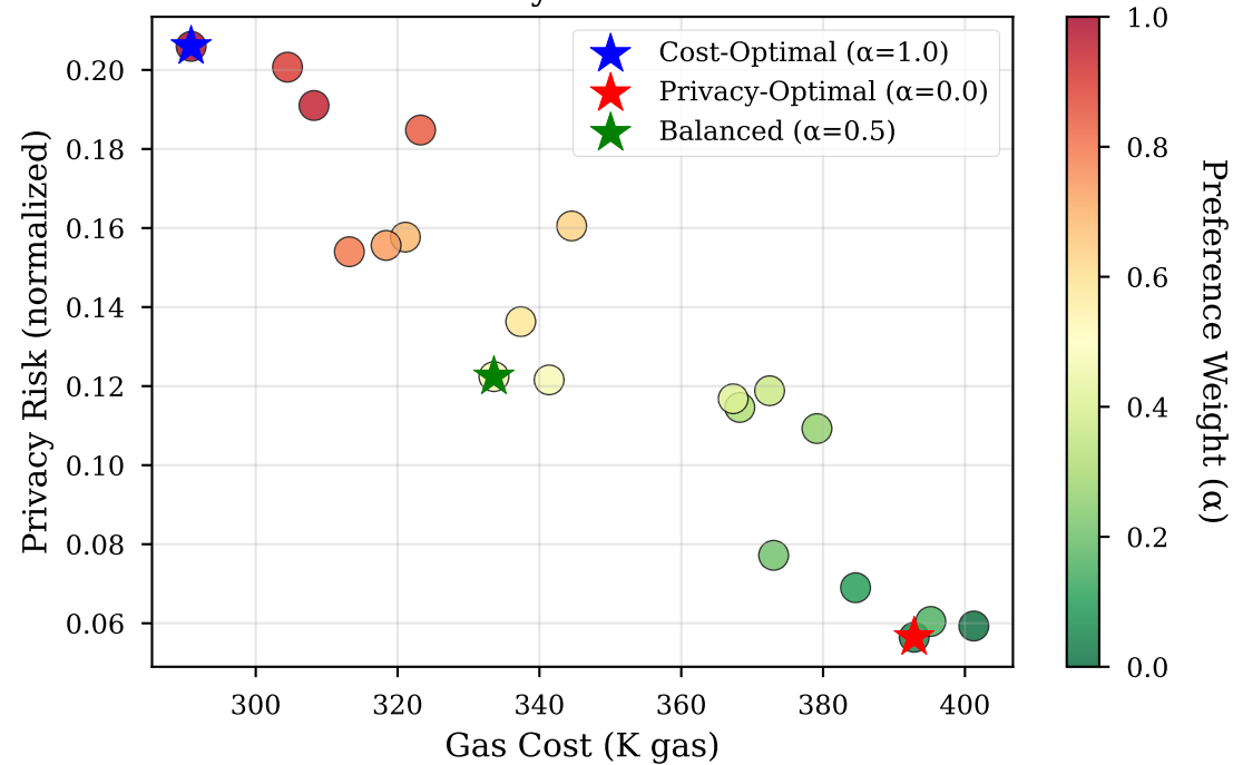
Cost-Privacy Pareto Frontier
