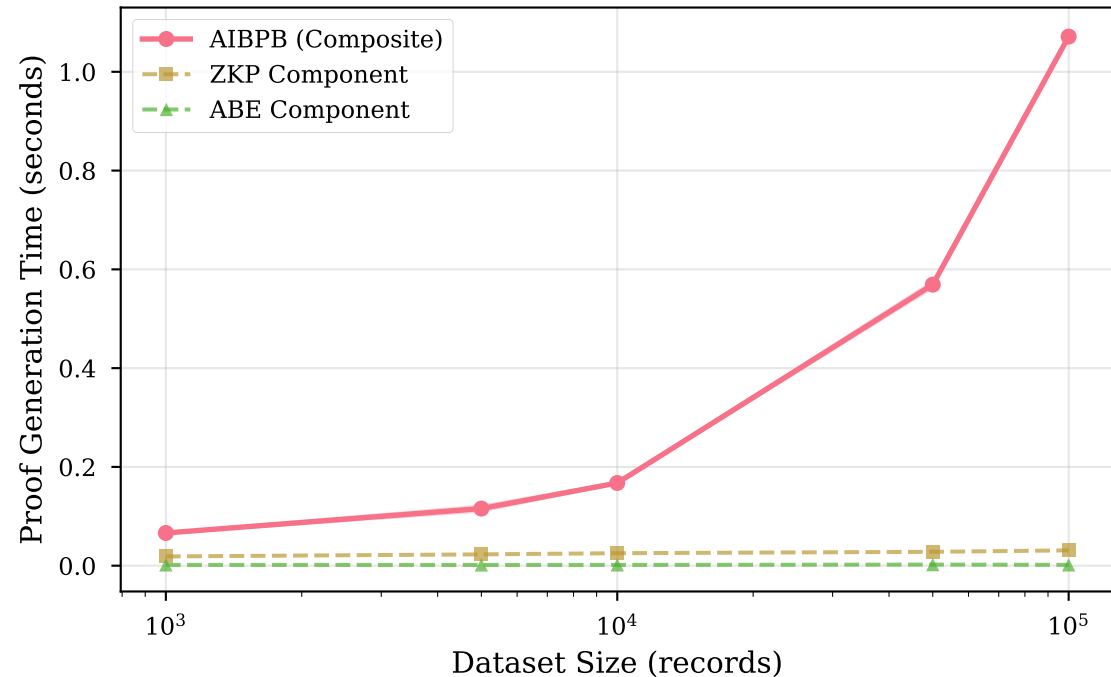
Proof Generation Time vs Dataset Size
