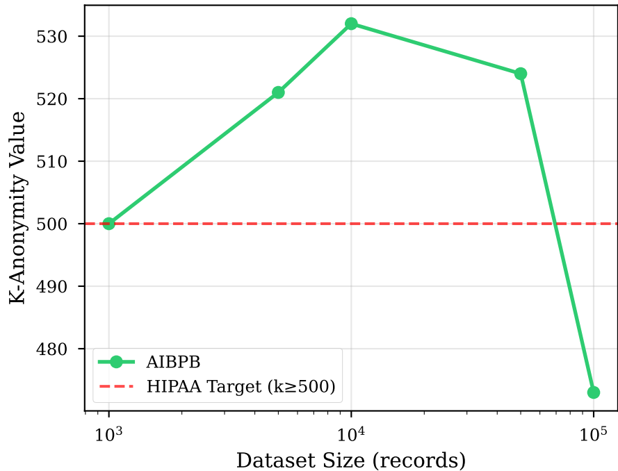
K-Anonymity Achievement
