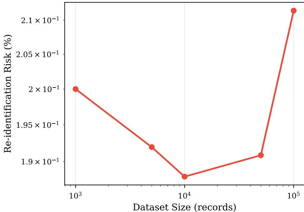
Re-identification Risk
