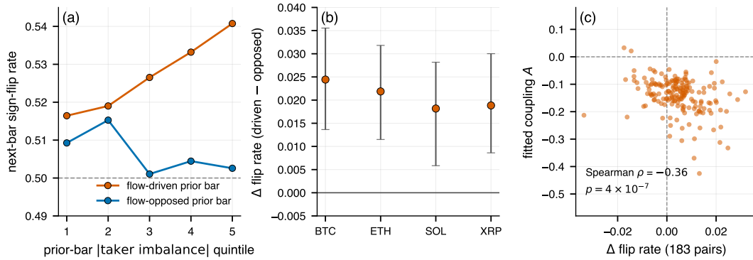
Figure 8: Reversal concentrates after flow-driven moves and grows with the flow. (a) Pooled next-bar sign-flip rate by quintile of the prior bar’s |taker imbalance| (four focal coins, 15 m, ~39k bars each), split by whether the prior move agreed with its flow: a dose-response after flow-driven bars, a coin-flip after flow-opposed ones. (b) The flow-driven minus flow-opposed flip-rate difference per coin with moving-block bootstrap CIs (pooled: +0.021, CI [0.015, 0.026]). (c) The conditioning scales to the cross-section: across the 183 pairs, those whose flow-driven moves revert harder carry systematically stronger fitted reversal couplings (three extreme-|A| pegged/microcap pairs outside the axis range).
