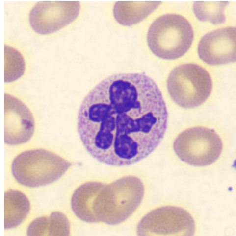
(a) Seg. neutrophil multi-lobed nucleus
