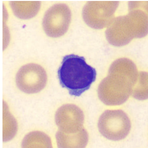
(b) Lymphocyte round dark nucleus
