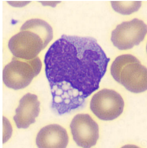
(c) Monocyte kidney-shaped nucleus
