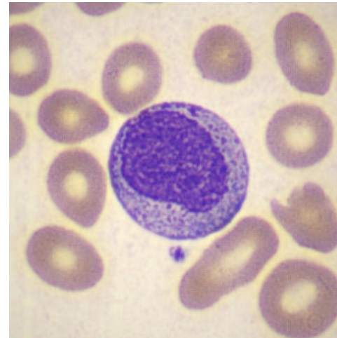
(e) Myelocyte round nucleus
