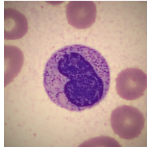
(f) Metamyelocyte indented nucleus
