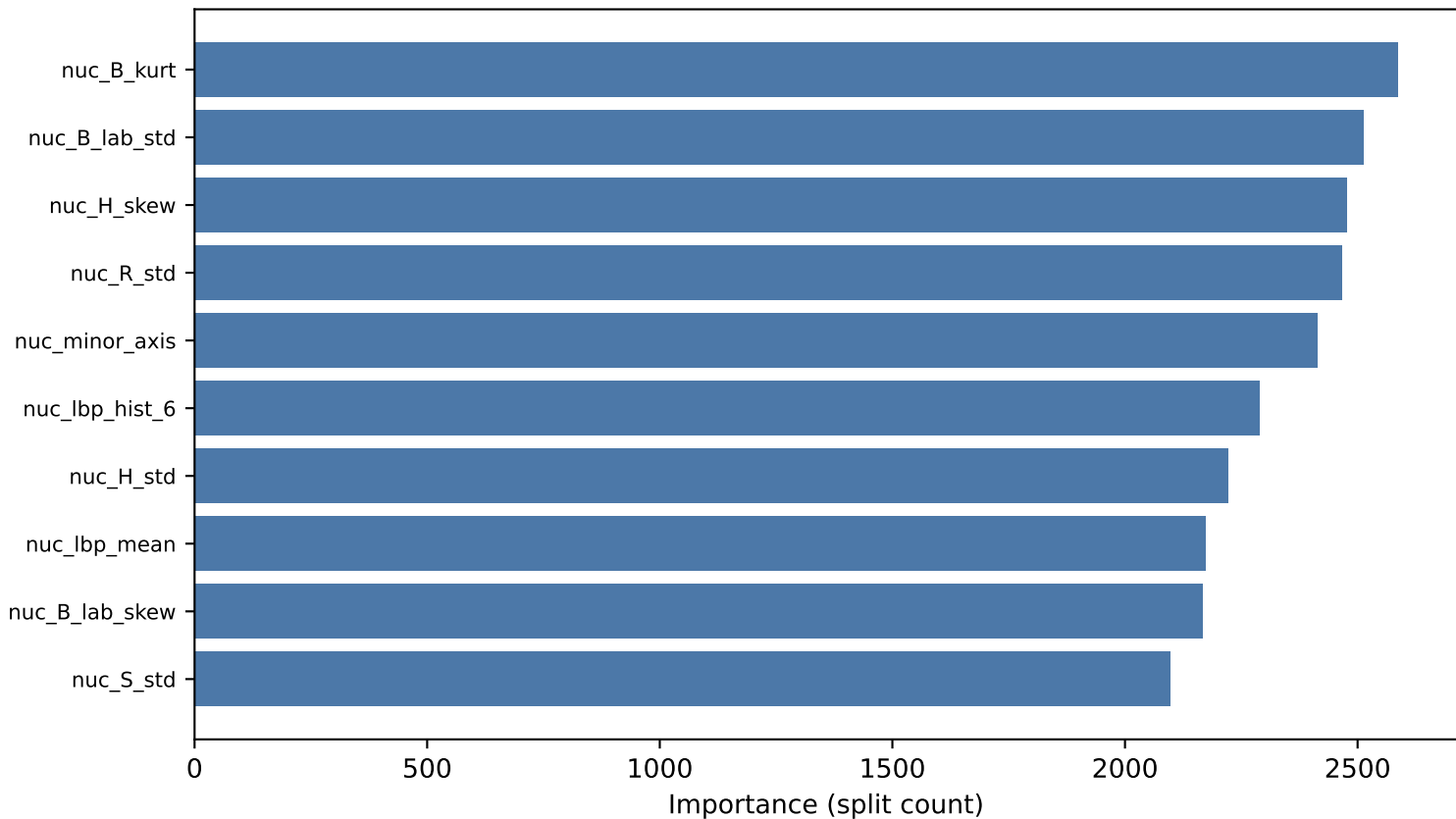
Top-10 handcrafted features (LightGBM split-count importance)
