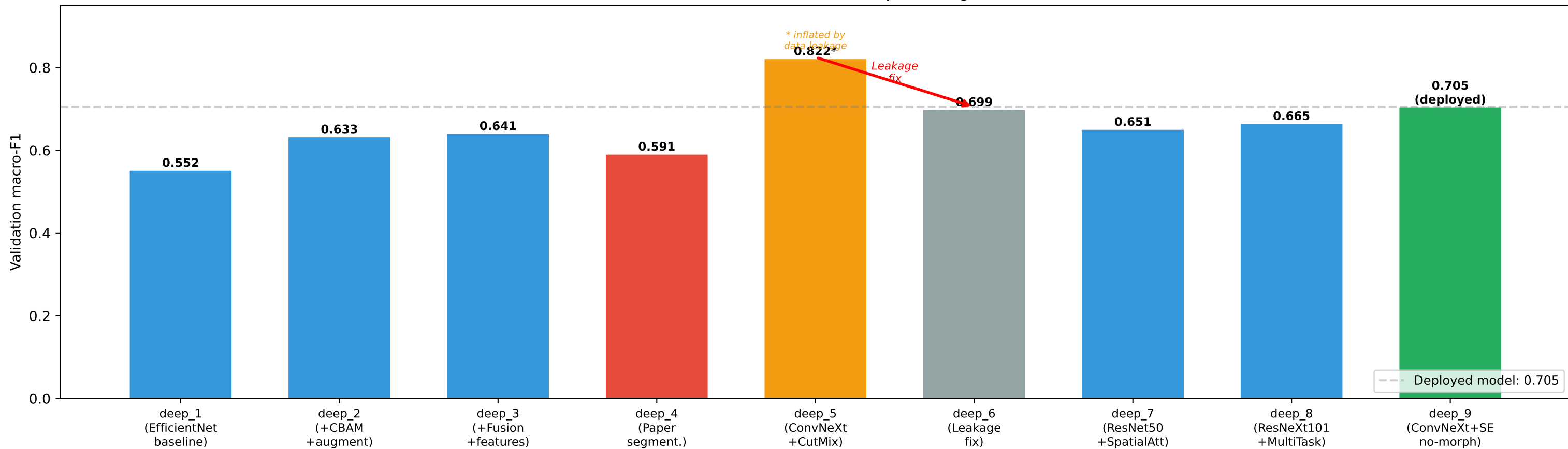
Validation macro-F1 across the 9 deep-learning iterations
