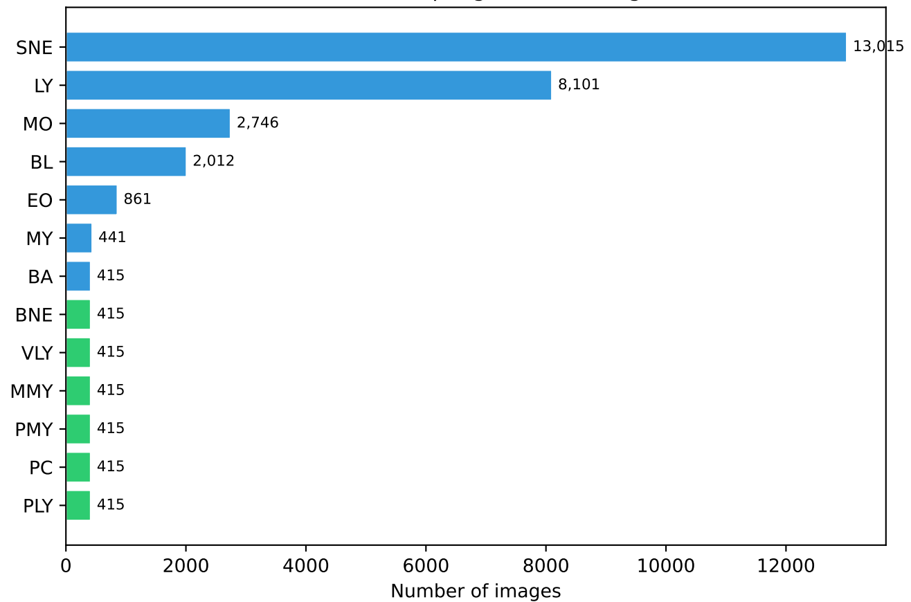
After oversampling (30,081 images)
