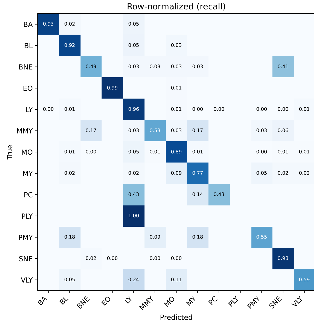
deep_9 no-morph, validation (n = 2,891), macro-F1 = 0.7052
