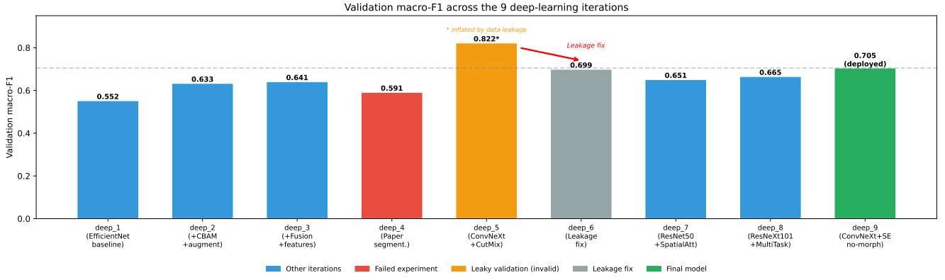
Figure 10: Validation macro-F1 across iterations. The deep 5 →deep 6 drop reflects the leakage correction, not a regression. Validation sets differ between deep 1 –deep 4 and deep 6 –deep 9 (see Table 6).
