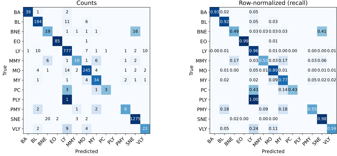
Figure 8: Confusion matrix (counts and normalized recall) of the final model.
