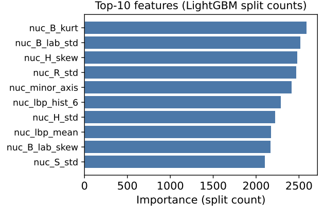
Figure 3: Top feature importances from LightGBM in Part I (split counts).
