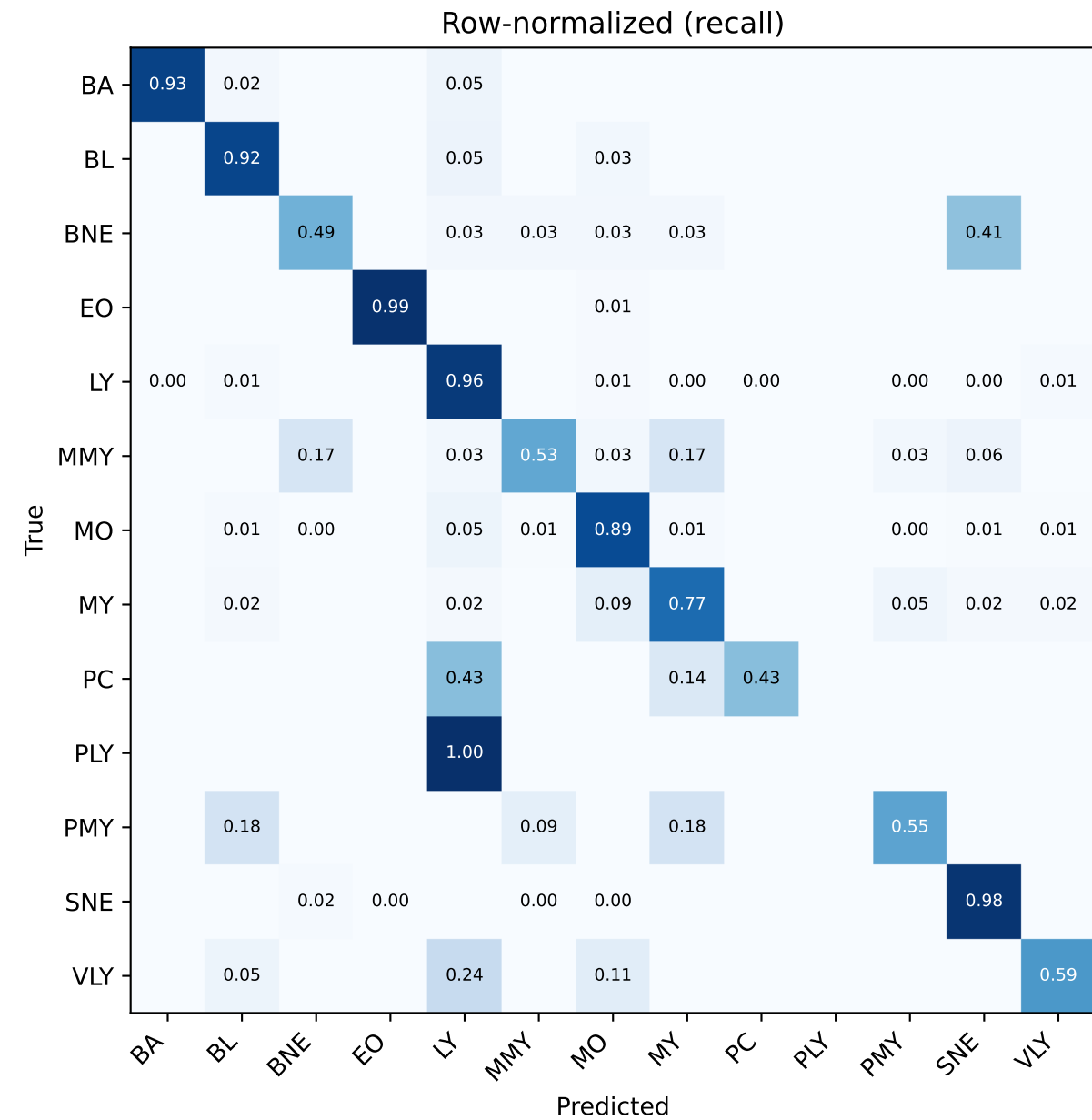
Final model, validation (n = 2,891), macro-F1 = 0.7052
