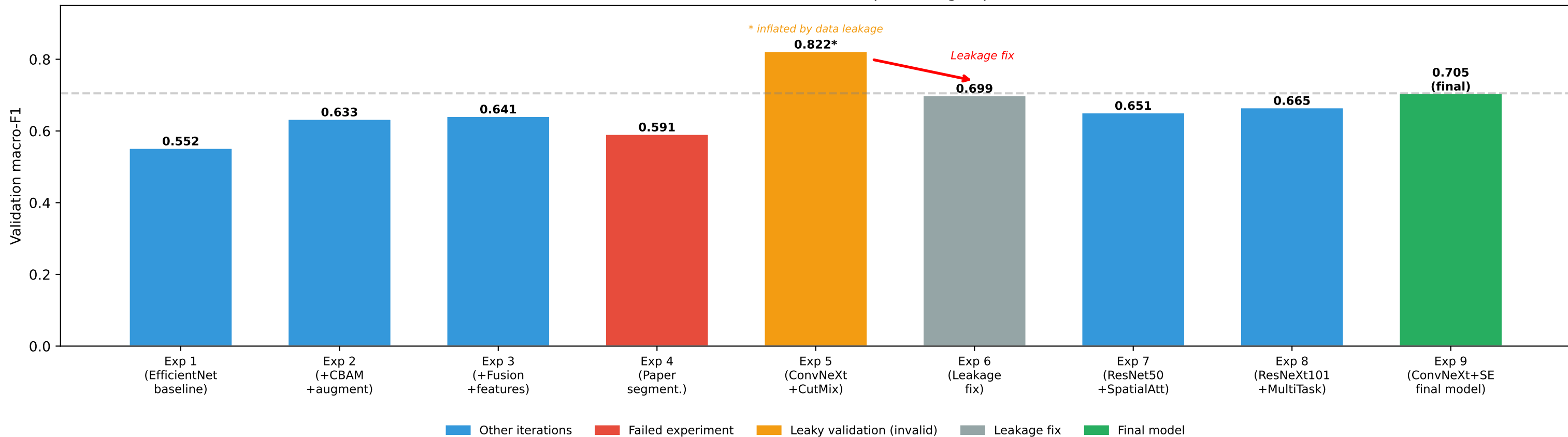
Validation macro-F1 across the 9 deep-learning experiments
