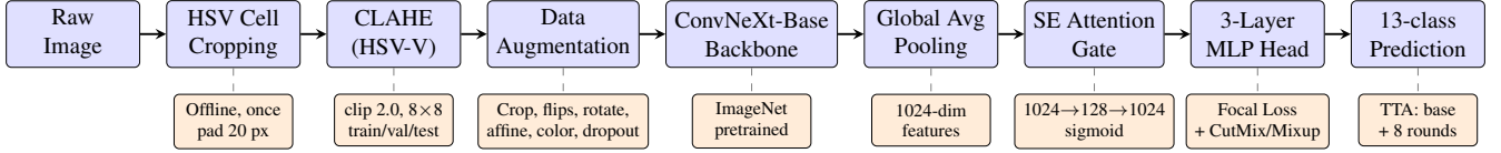
Figure 4: Final deep learning pipeline. HSV cropping removes background distractors, CLAHE equalizes local contrast, augmentation builds geometric and photometric robustness, ConvNeXt-Base learns hierarchical features, a lightweight attention gate reweights them, and Focal Loss handles class imbalance.
