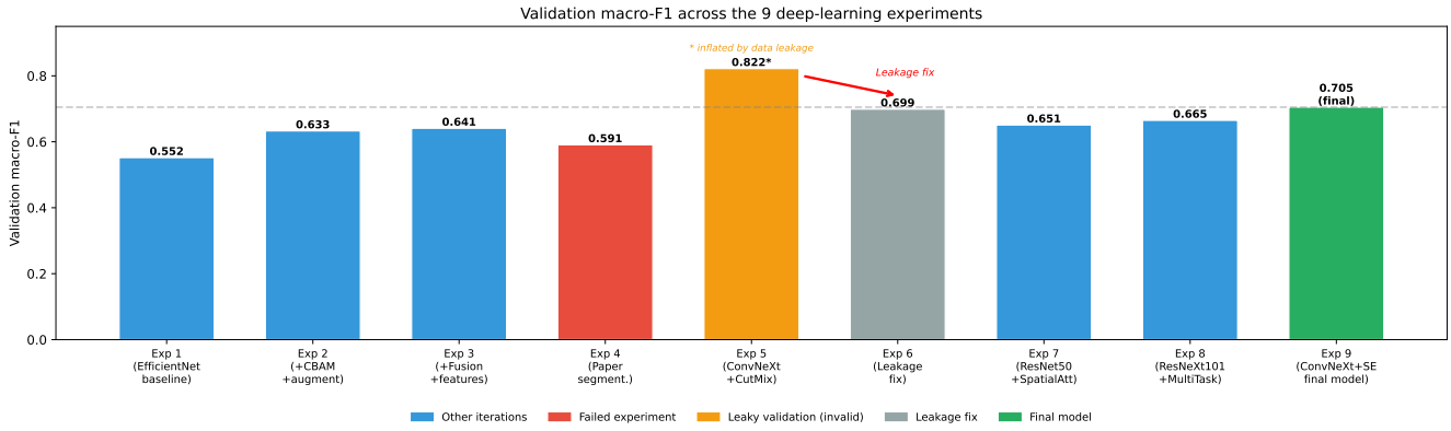
Figure 10: Evolution of validation macro-F1 across experiments. The drop from Exp 5 to Exp 6 reflects the leakage correction, not a regression. Validation sets differ between Exp 1–4 and Exp 6–9 (see Table 6).
