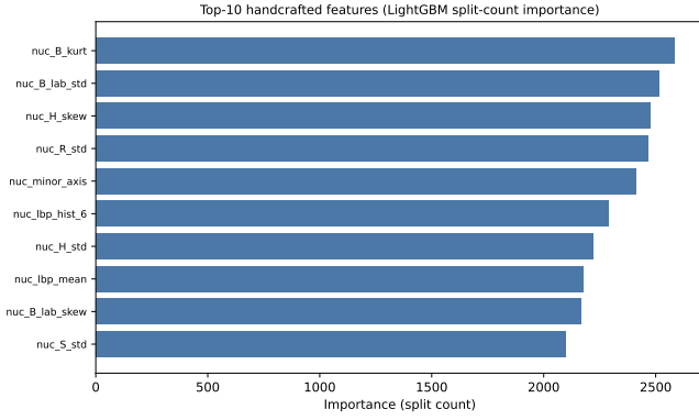
Figure 3: Top feature importances from LightGBM in Part I (split counts).
