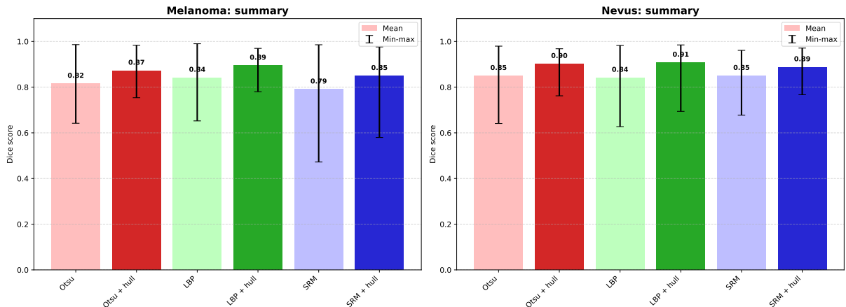
Figure 5: Mean Dice per method with min–max whiskers, melanoma (left) and nevus (right). SRM’s spread is much wider on melanomas, down to 0.47 on ISIC_0000049; Otsu’s is similar on both, and LBP’s is wider on nevi, where ISIC_0000095 pulls it down.
