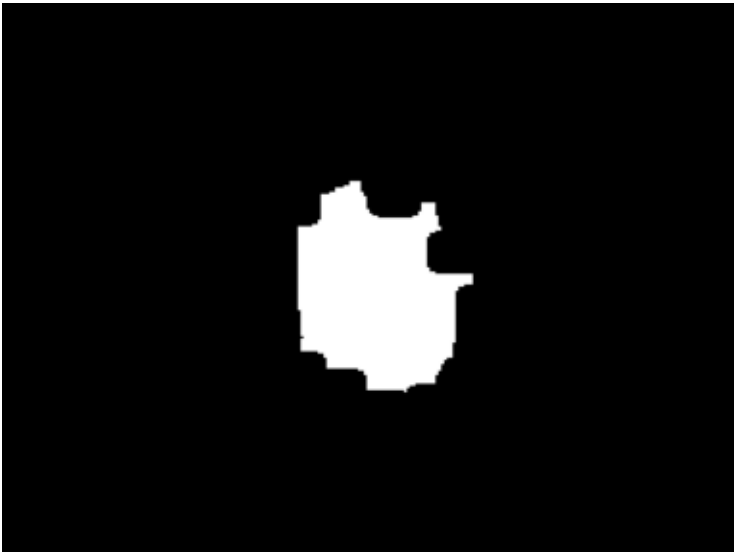
SRM Dice 0.863
