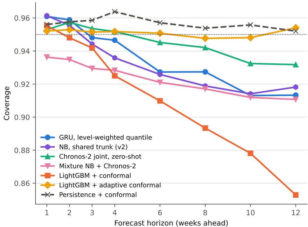
Empirical coverage of the 95% interval (target 0.95)
