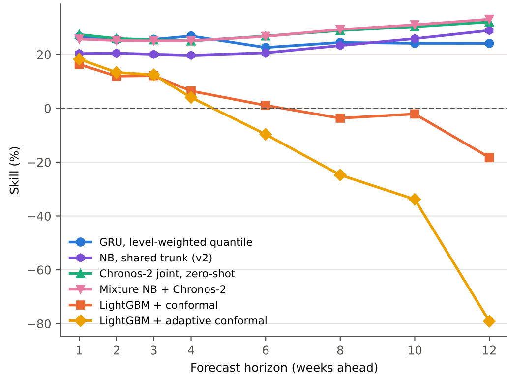
WIS skill vs persistence with conformal intervals
